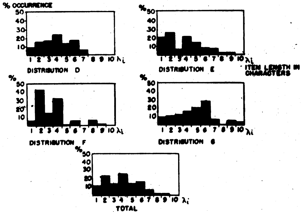
Numerical Item Lengths in Four Payrolls
