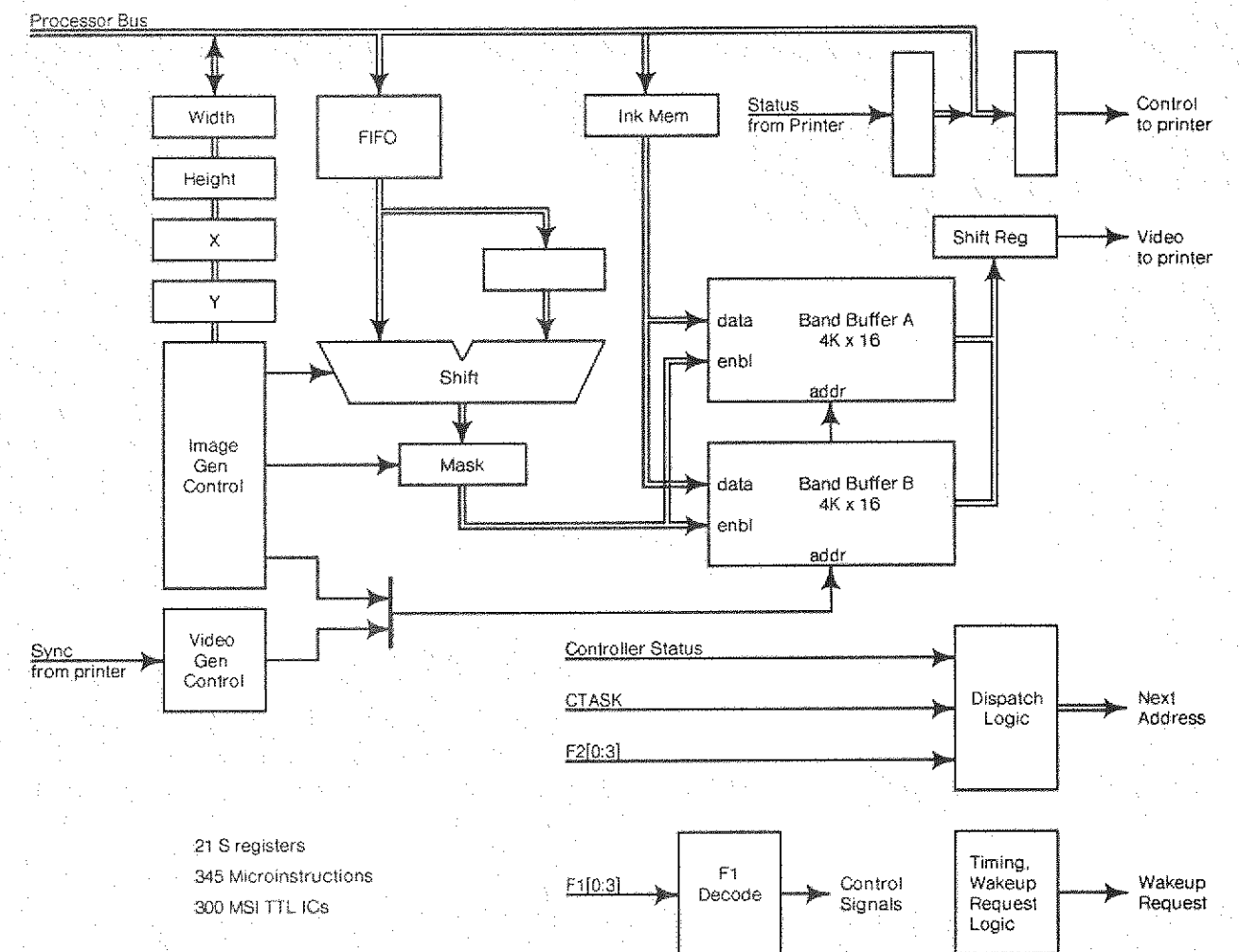
Figure 14. The printer controller.
