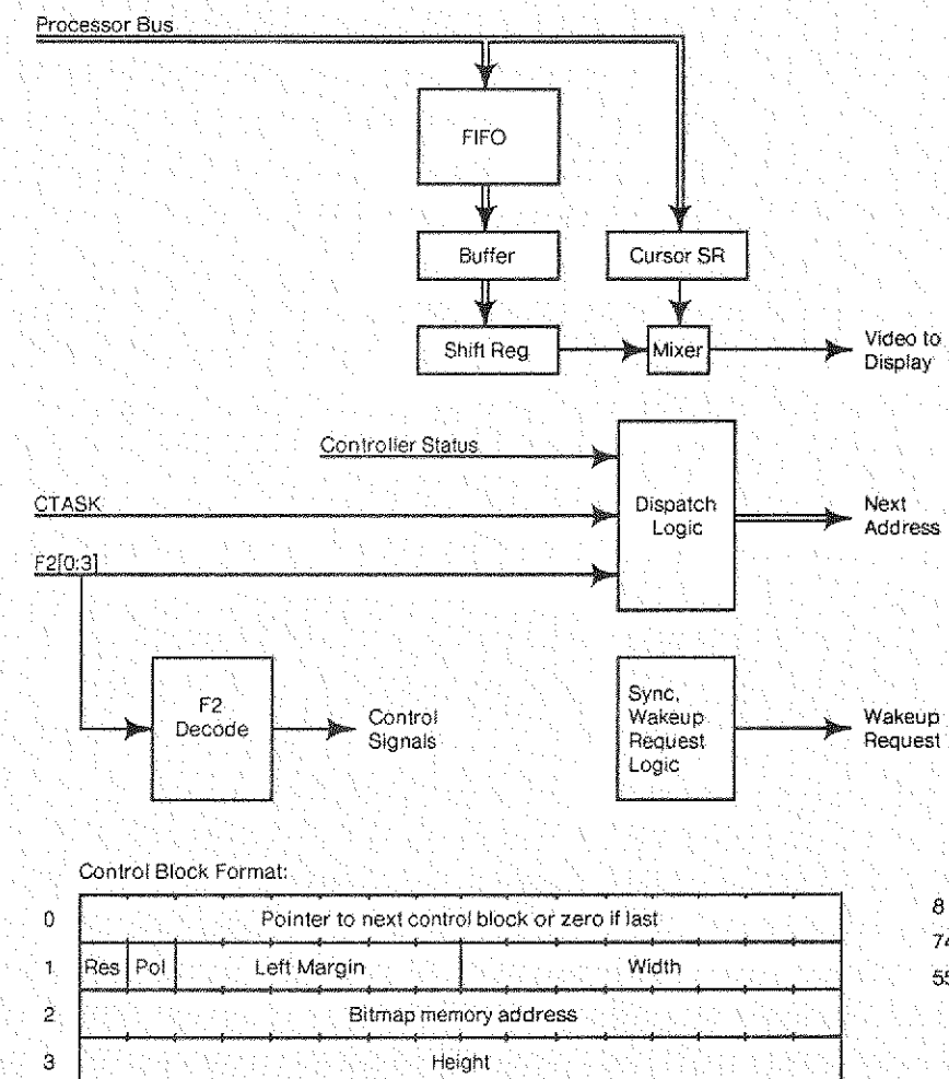
Figure 9. The display controller.
