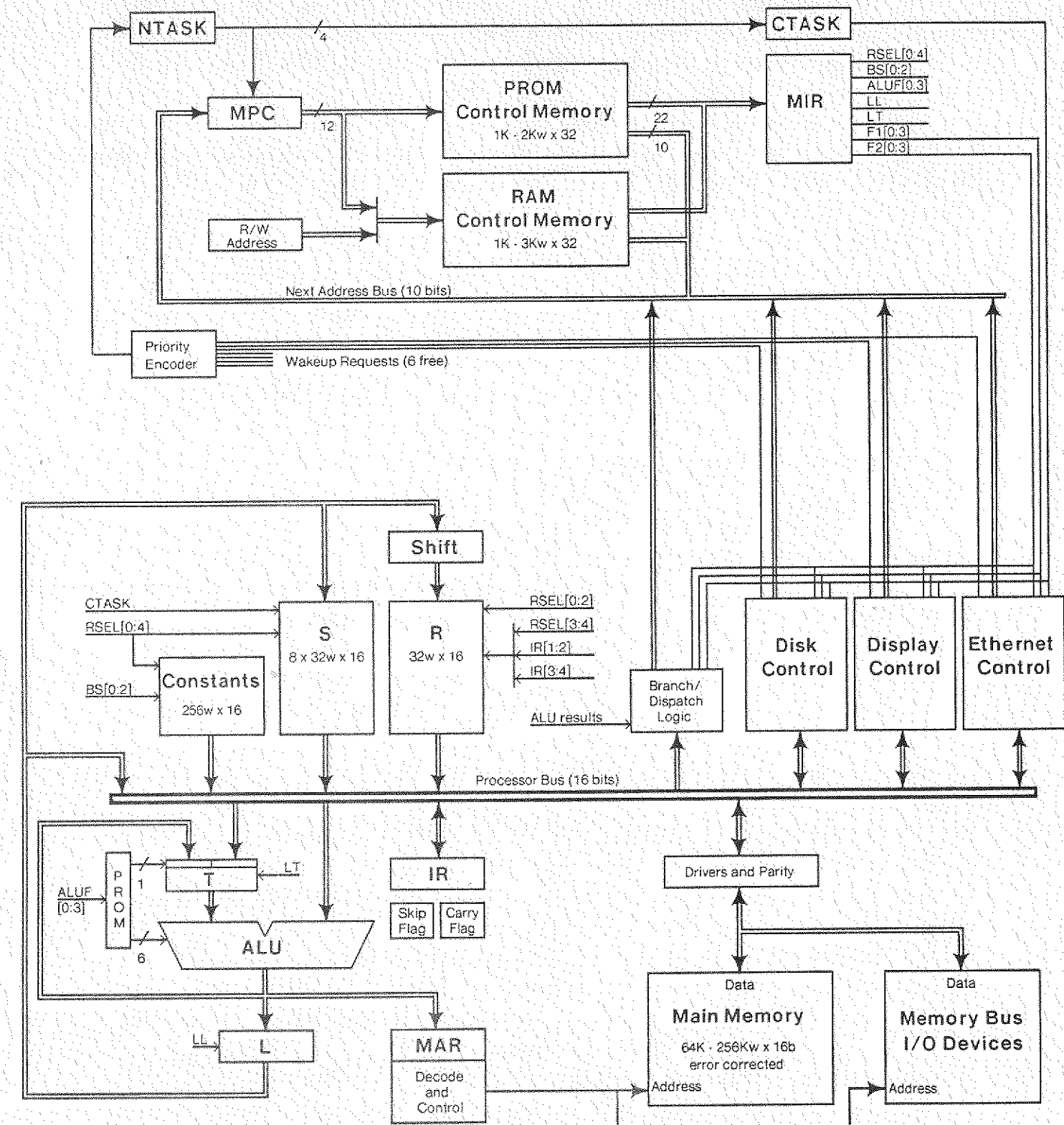
Figure 6. Alto micromachine structure.
