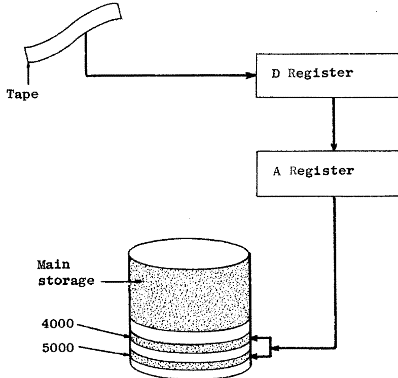
Figure V. Information path during magnetic tape READ.
