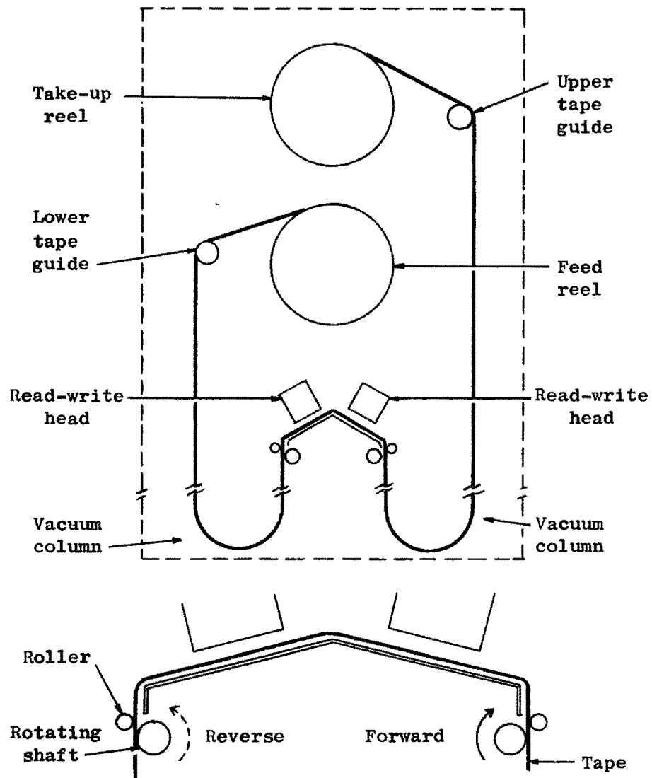
Figure II. Tape movement.
