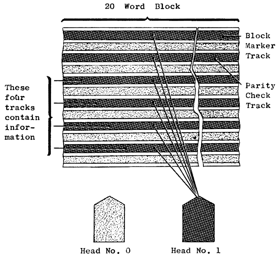
Figure 1. Tape detail.
