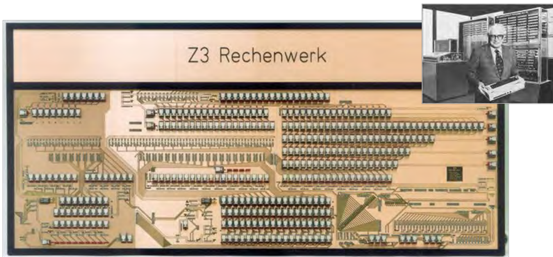
Figure 5. Reconstruction of Konrad Zuse's Z3 (part). Front view of processor.
