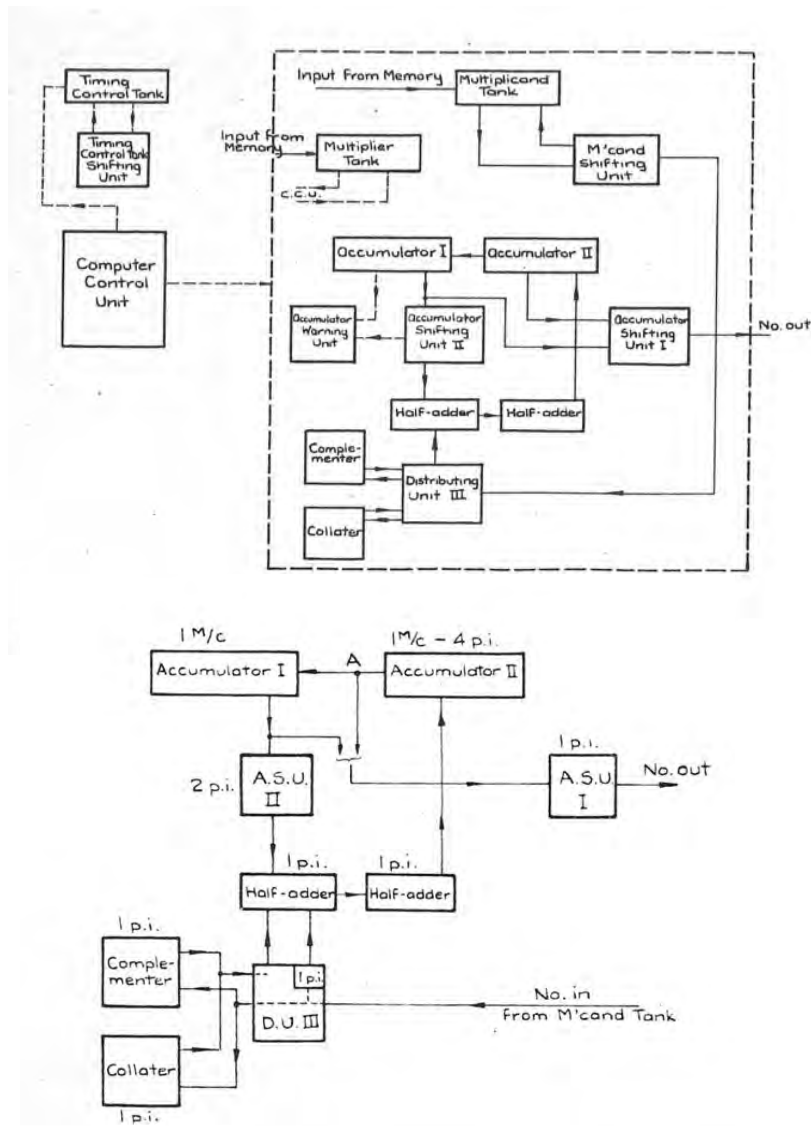
Fig.13. DELAYS IN COMPUTER
