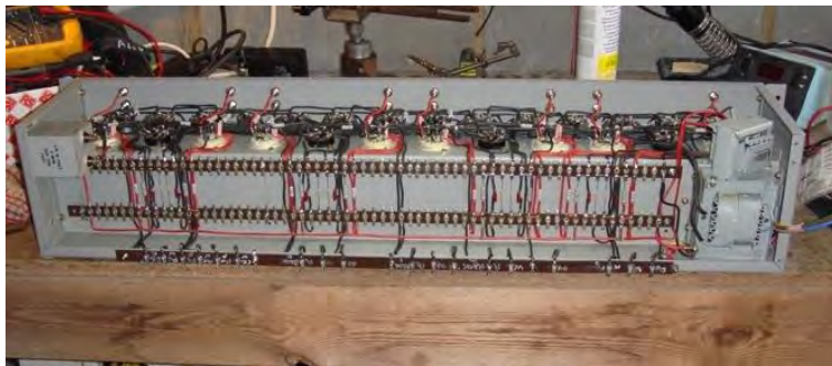
Figure 8. Original versus replica chassis
