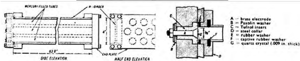
Figure 1. Photograph and drawings of the long mercury tanks
