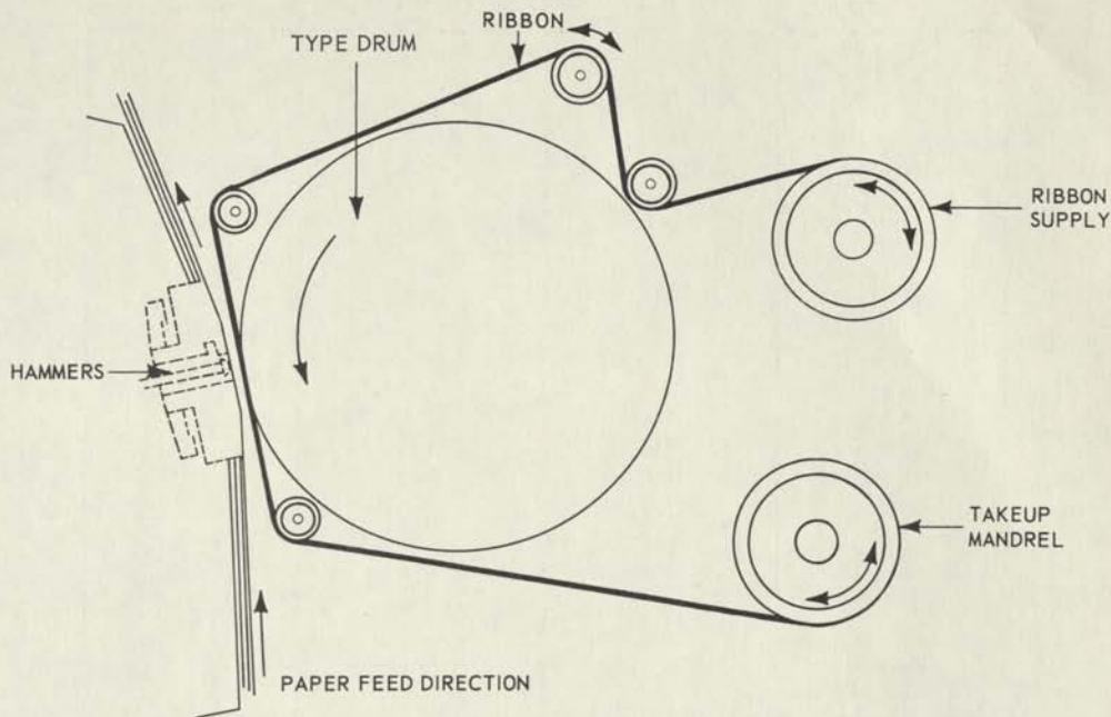
Figure 2-3. Printer Mechanism
