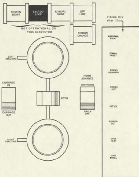
Figure 4-2. Right-hand Control Panel
