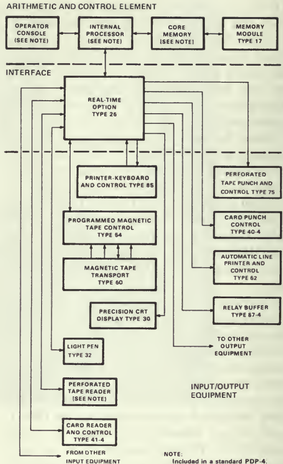
Figure 16. PDP-4 block diagram.
