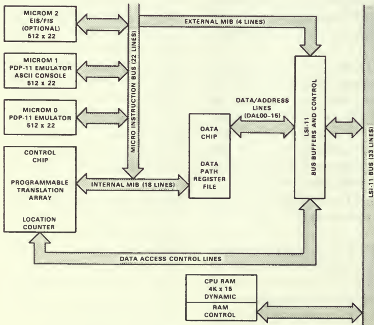
Figure 2. Organization of the LSI-11 CPU.
