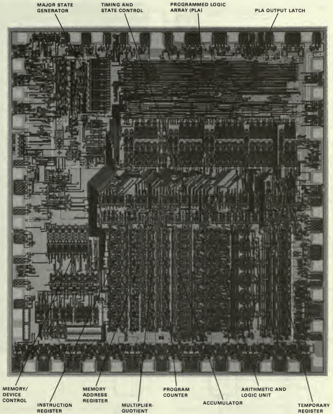
Figure 17. Microphotograph of the CMOS-8 chip (courtesy of Intersil Corporation).
