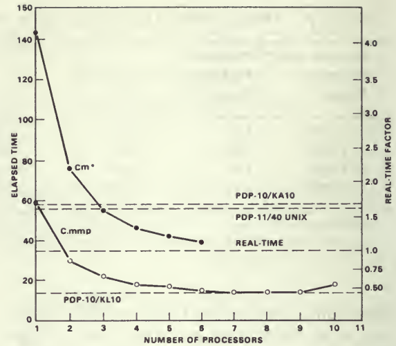
Figure 5. A performance comparison of two multiprocessors, C.mmp and Cm*, with three uniprocessors at Carnegie-Mellon University. The application used is HARPY, a speech recognition program.
