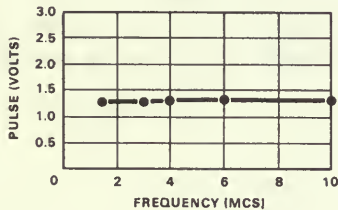
Figure 10. Trigger sensitivity.
