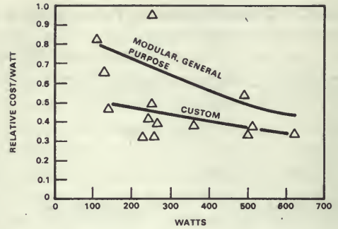
(a) Cost efficiency (in relative cost per watt).
