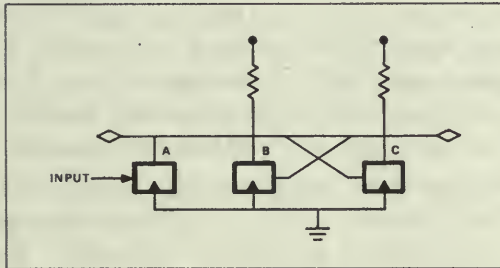
Figure 10. Primitive flip-flop with inverter.
