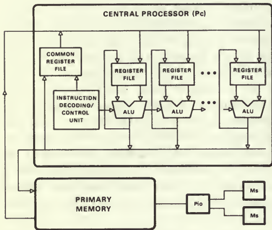
Figure 4. Multi-ALU processor.
