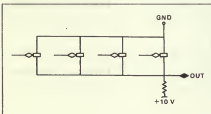
Figure 4. Parallel inverters.
