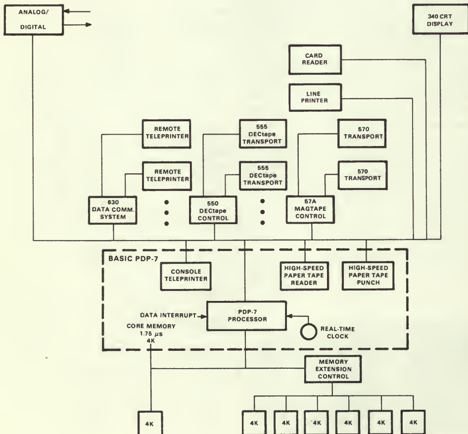
Figure 22. PDP-7 system block diagram.
