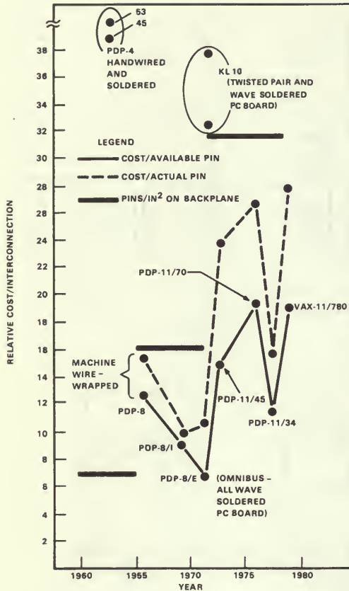
Figure 12. Relative cost per possible and actual interconnection versus time for various DEC computer backplanes; also pin density (in pins per in 2 ) versus time.
