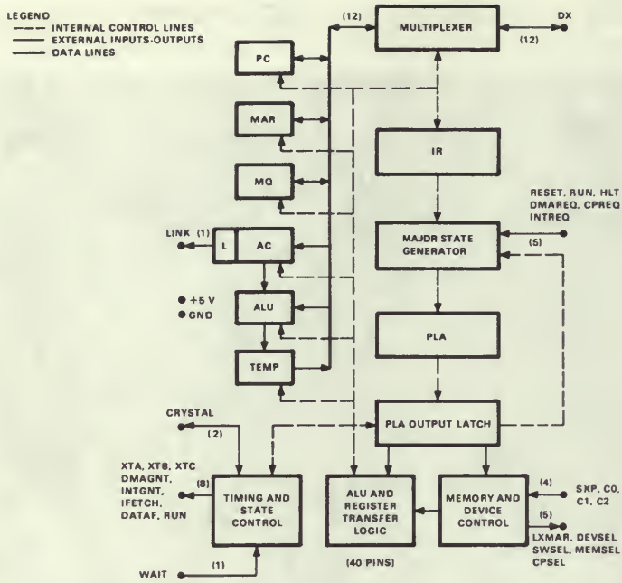
Figure 18. Block diagram of CMOS-8.
