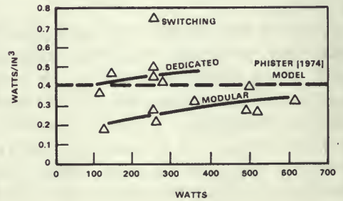
(c) Volumetric efficiency (in watts per in³).
