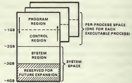
Figure 8. Virtual address space.
