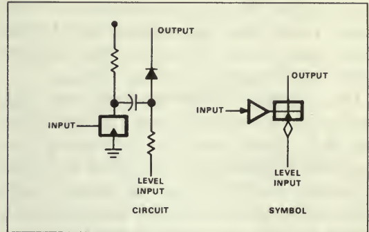
Figure 13. Positive C-D gate.
