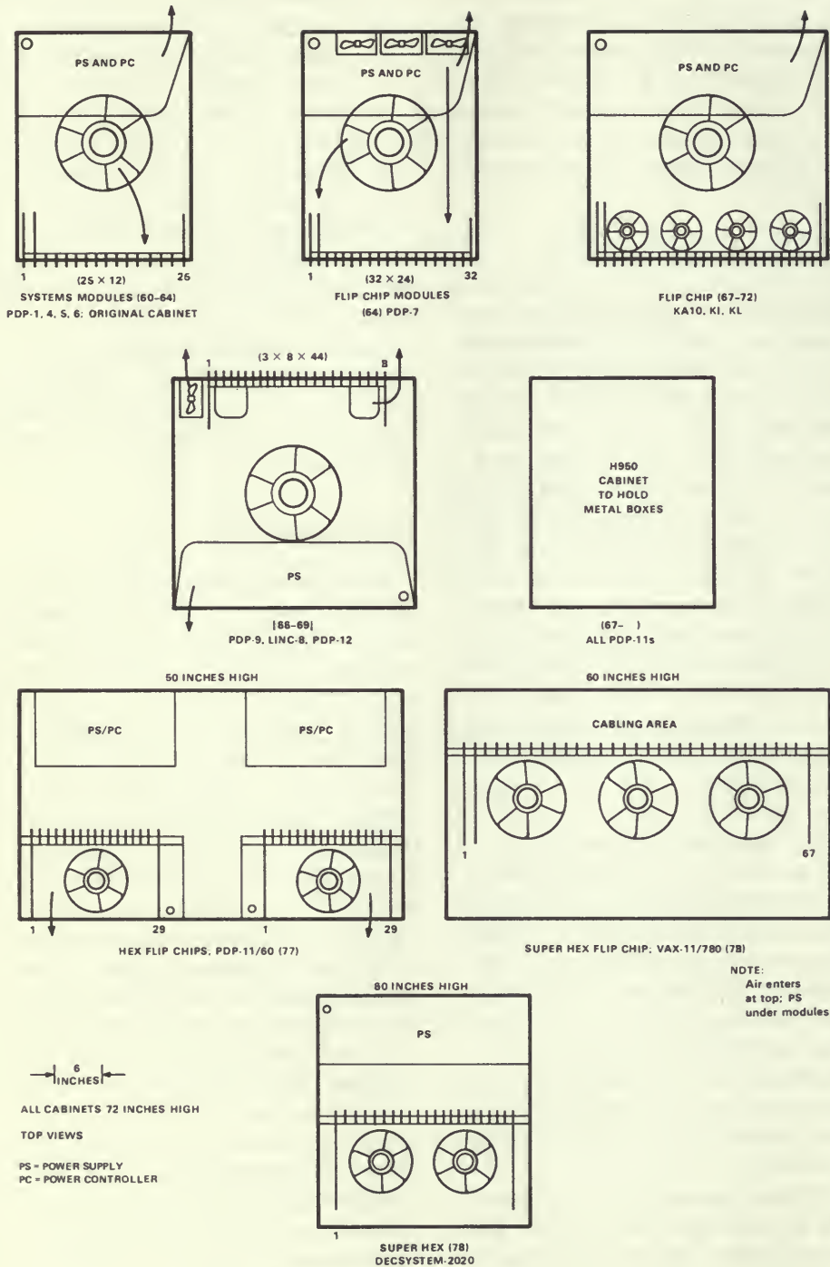
Figure 10. Cabinets used to hold various DEC computers (in fixed, book, and box configurations).
