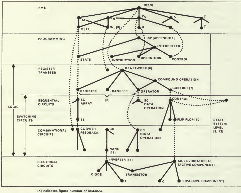
Figure 1. PDP-8 hierarchy of descriptions.
