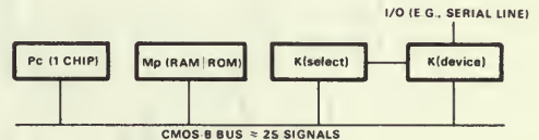
(c) CMOS-8 (6100) processor-on-a-chip family.
