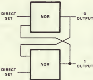
(b) Combinational logic equivalent of flip-flop.
