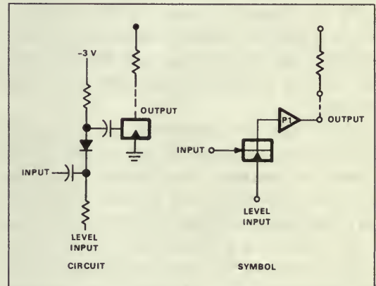
Figure 14. Negative C-D gate.
