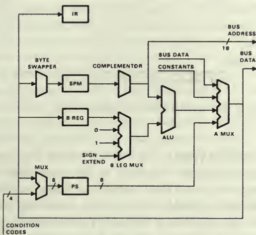
Figure 8. PDP-11/04 data paths.
