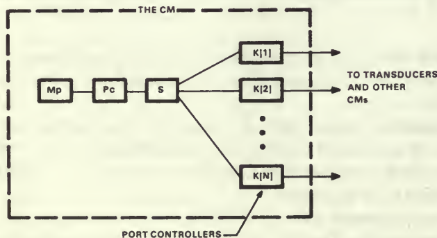
Figure 2. PMS diagram of Computer Module.
