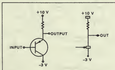
Figure 1. Emitter follower.
