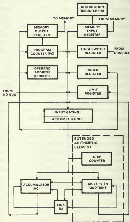
Figure 31. PDP-15 processor register transfer diagram.
