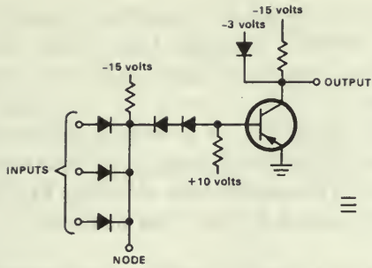
(a) Multiple input inverter circuit.
