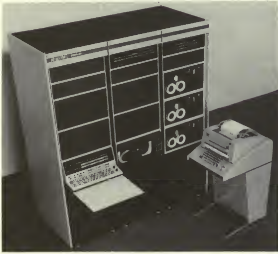
Figure 29. PDP-15/10.
