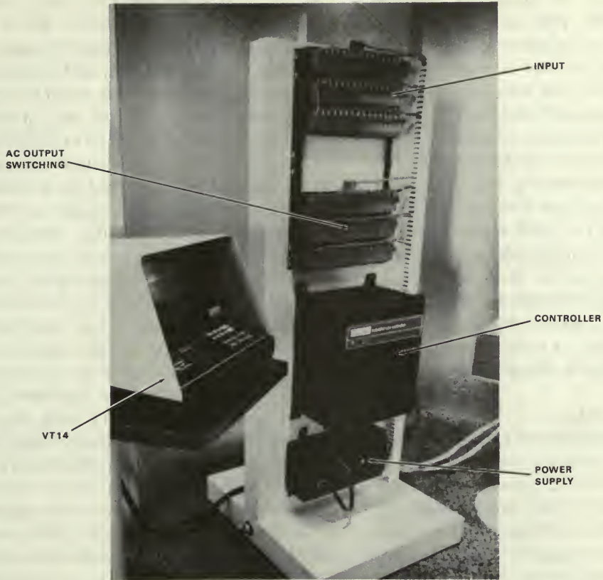
Figure 34. The PDP-14/30.
