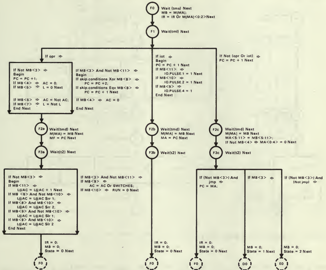
Figure 7. PDP-8 Pc state diagram (part 1 of 2).
