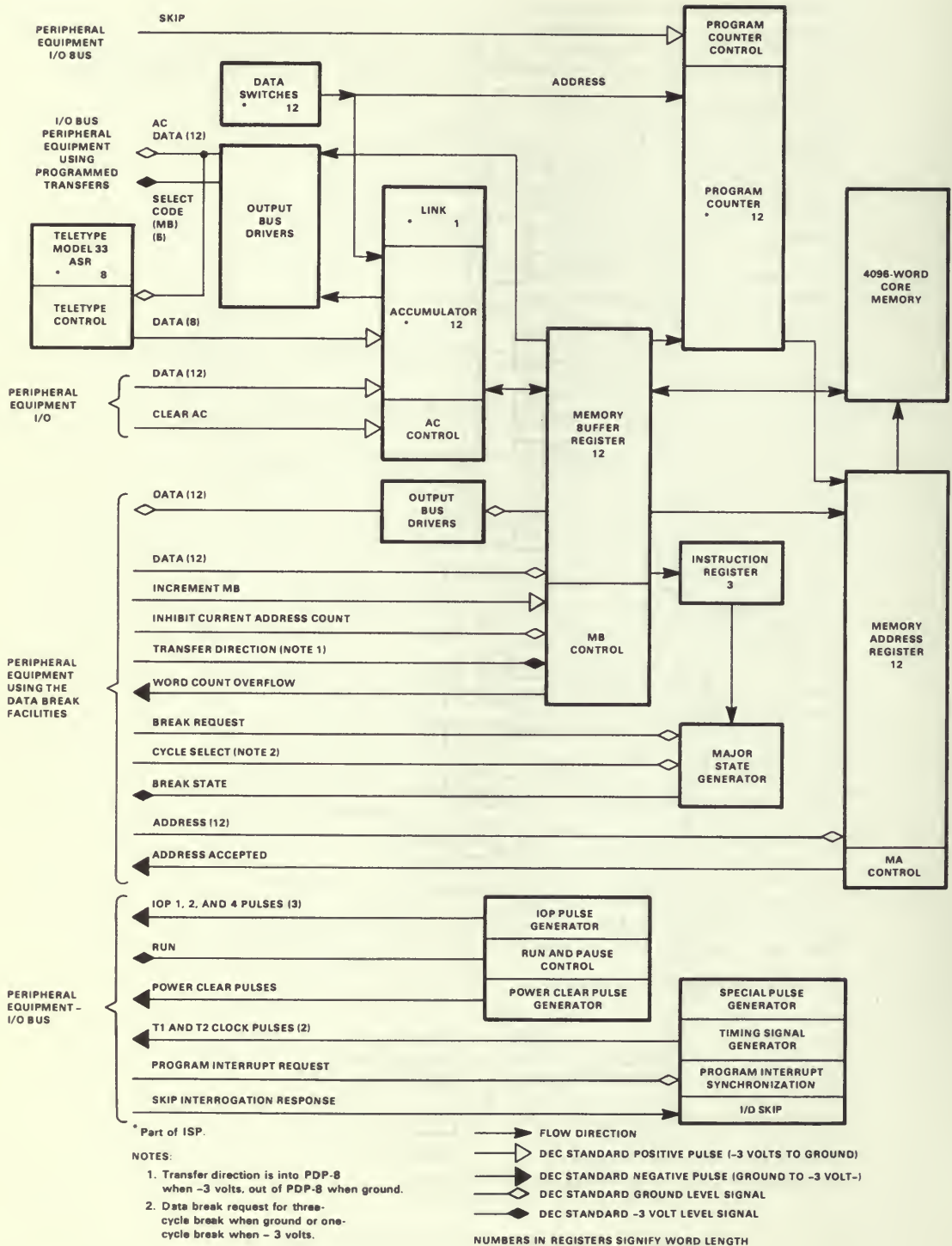
Figure 4. PDP-8 processor block diagram.
