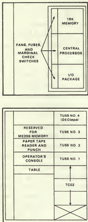
Figure 27. PDP-9 front and back logic layout.
