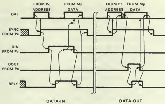
Figure 20. LSI-11 Bus Data-In and Data-Out synchronization.
