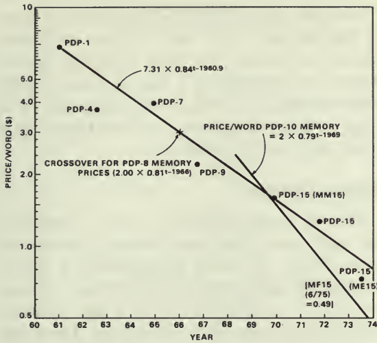
Figure 36. Price/word of 18-bit memory versus time.
