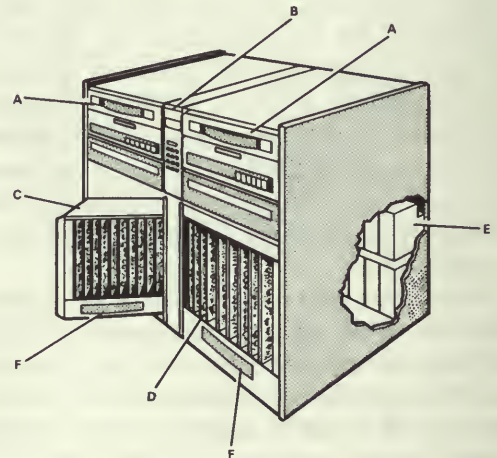
LEGEND: A - DISK DRIVES B - MAINTENANCE CONSOLE C - CARD CAGE SWUNG INTO MAINTENANCE-ACCESS POSITION D - CARD CAGE IN CLOSED POSITION E - REAR ACCESS MODULAR POWER SUPPLIES F - BLOWER SYSTEM
