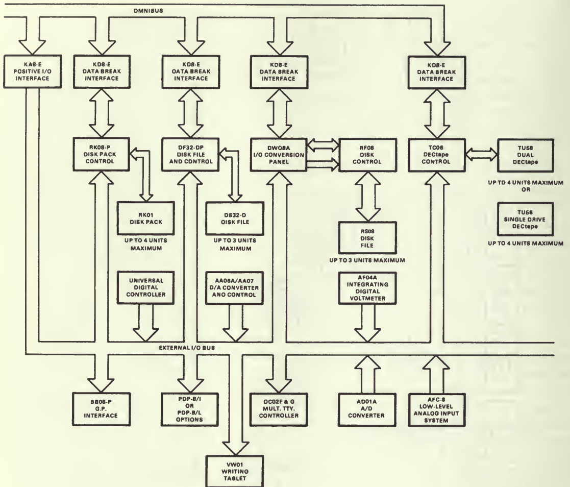
Figure 12. PDP-8/E system block diagram (part 2 of 2).
