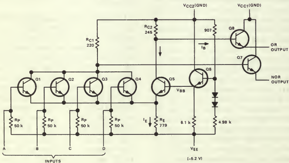
Figure 21. ECL circuit.
