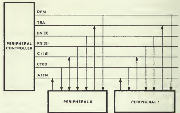
Figure 25. The Control Section signals of the Massbus.
