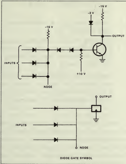
Figure 17. Diode gate.
