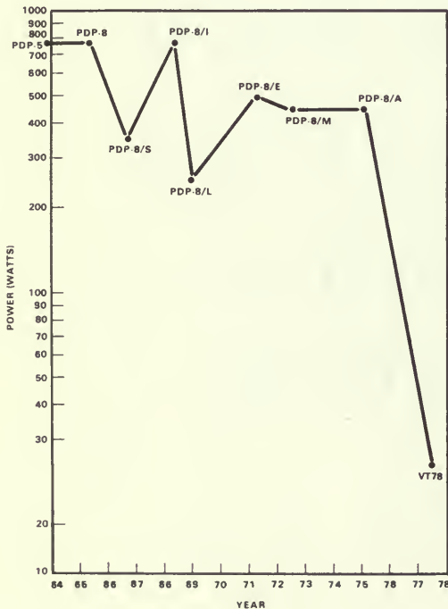
(a) Power versus time.
