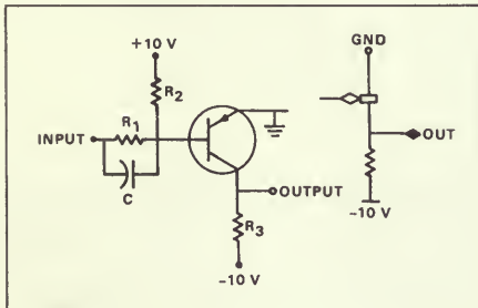
Figure 3. Inverter.
