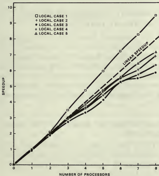
Figure 21. Integer programming speedup.
