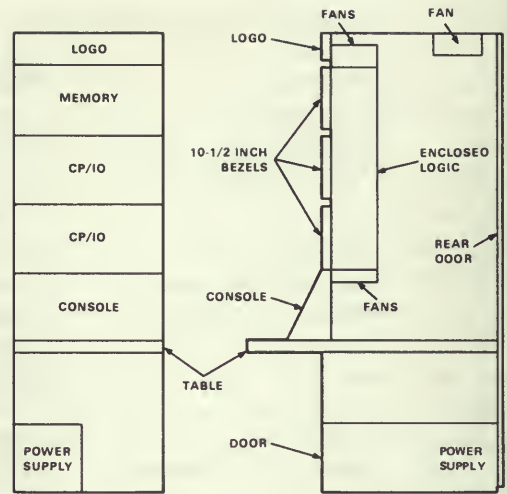
DEC 19-INCH CABINET DIMENSIONS: 30 INCHES DEEP; 21-11/16 INCHES WIDE; AND 71-7/16 INCHES HIGH.
