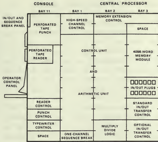
Figure 13. PDP-1/C logic layout diagram.
