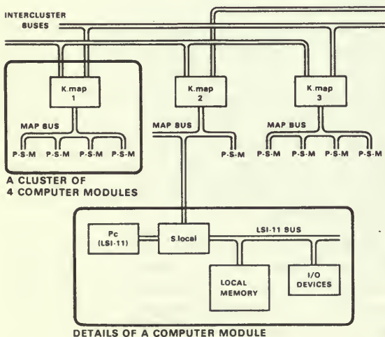
Figure 6. The basic structure of Cm*
