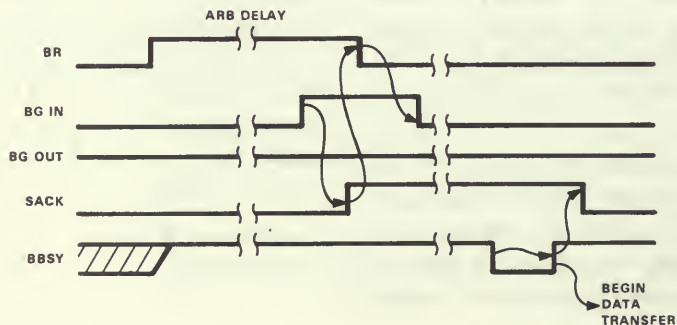
Figure 13. The timing of a Unibus arbitration sequence.
