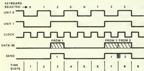
Figure 17. Timing diagram of a polled character-input bus.
