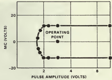
Figure 16. Pulse margins.
