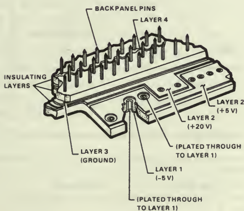
Figure 5. Cross-section of a printed circuit backplane.
