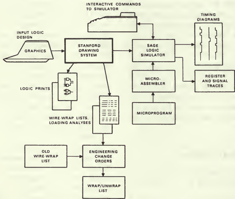
Figure 7. CAD system at CMU.
