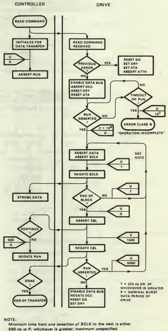
Figure 2. The Data Read flowchart in the Massbus specification.
