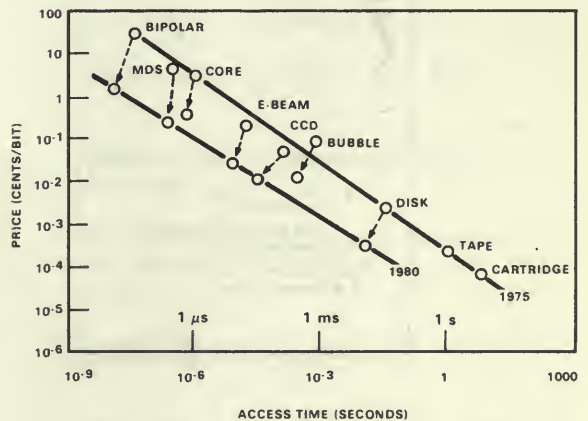
Figure 17. Memory trends, 1975–1980 (courtesy of Memorex Corporation, 1978).
