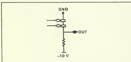
Figure 5. Series inverters.
