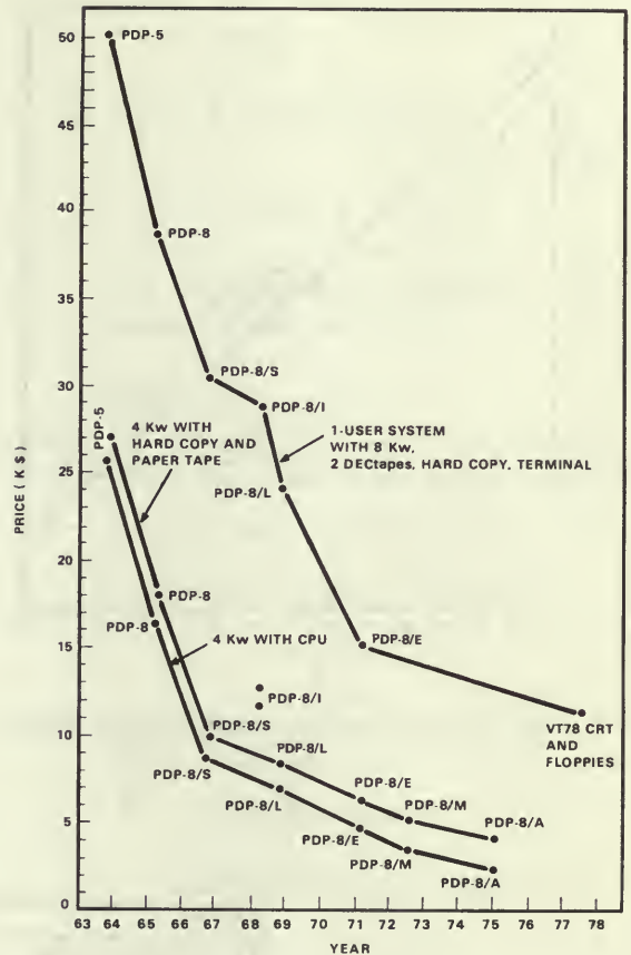
Figure 24. Price of DEC's 12-bit computers versus time (linear).
