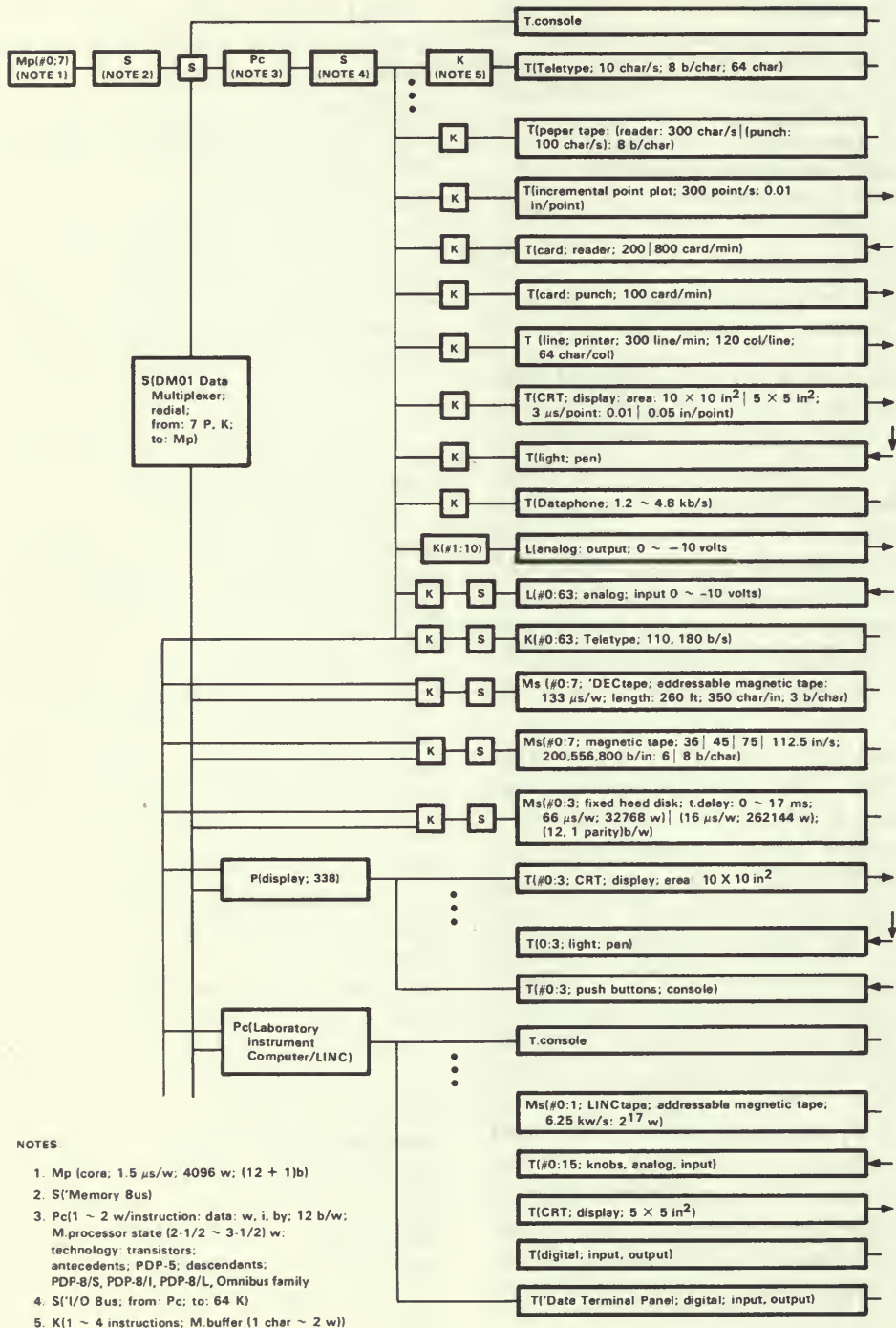
Figure 2. LINC-8-338 PMS diagram.
