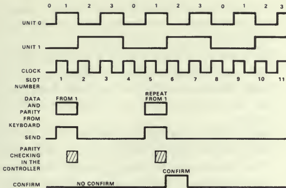
Figure 32. Timing of a plausible error-checking scheme with acknowledgement and retry for polled character-input bus.
