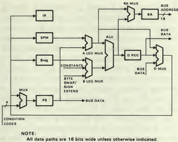
Figure 6. PDP-11/40 data paths.
