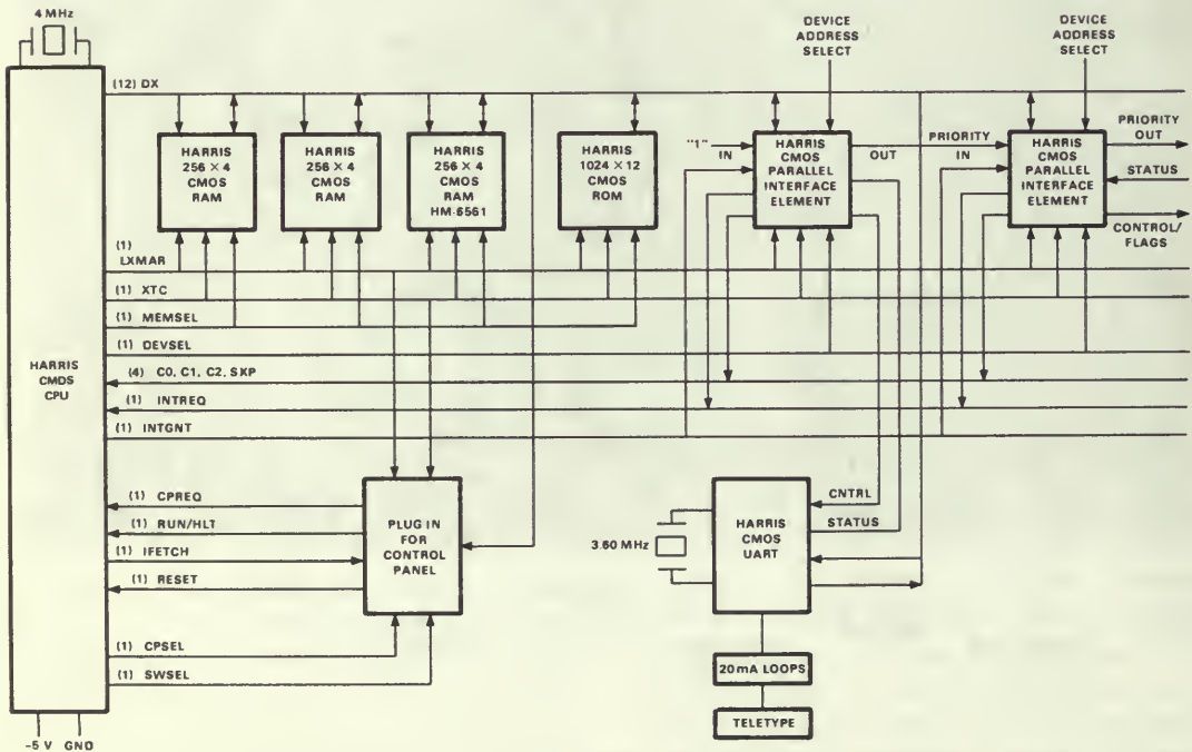
Figure 19. CMOS-8 based system.
