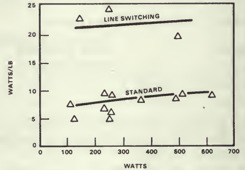
(b) Weight efficiency (in watts per lb).
