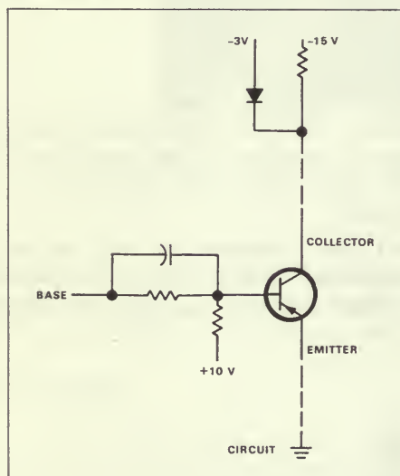
Figure 3. Schematic drawing of an inverter used in digital system modules.
