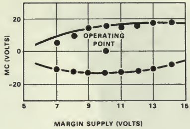
Figure 13. -10 V supply margins.
