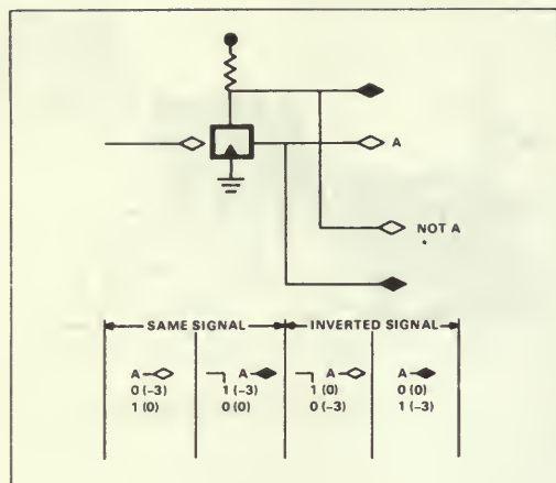
Figure 6. Signal naming convention for DEC dual polarity logic.
