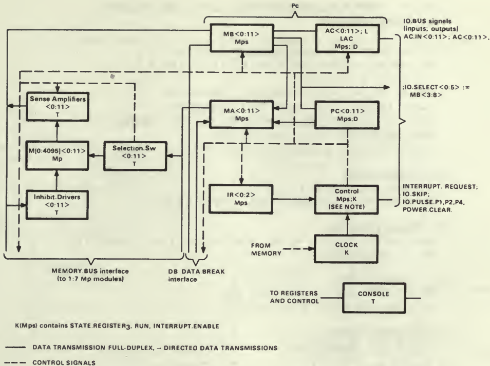
Figure 6. PDP-8 register transfer level PMS diagram.
