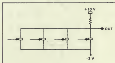
Figure 2. Parallel emitter follower.
