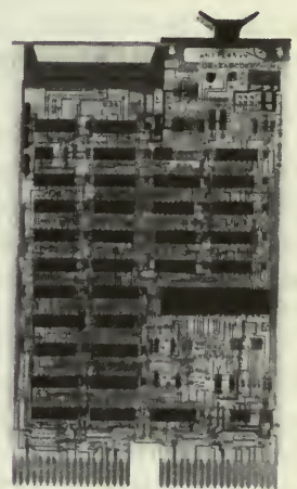
DLV11 Single-line serial interface
