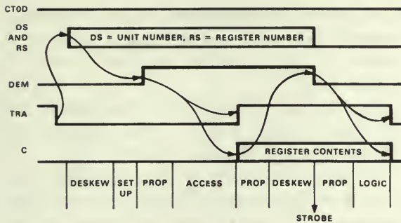
Figure 26. Timing of a control read in the control section of the Massbus.
