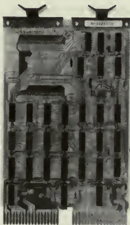
REV11-A Refresh/ bootstrap/ diagnostic/ terminator module
