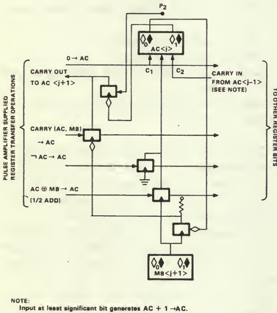
Figure 12. Logic diagram of PDP-1 Accumulator bit, AC<j> .
