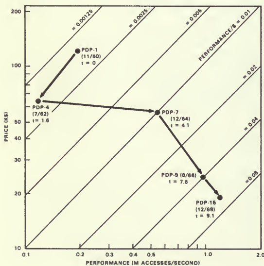
Figure 39. Price versus performance of 18-bit machines.
