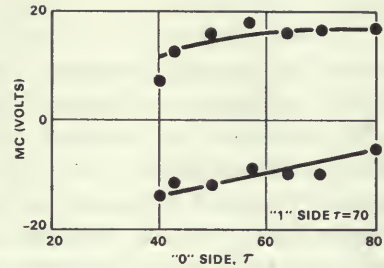
Figure 11. Tau margins.
