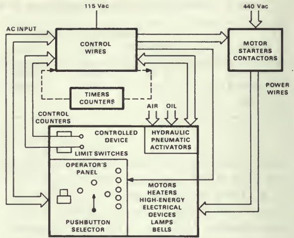
Figure 31. Hardwired machine for industrial control.
