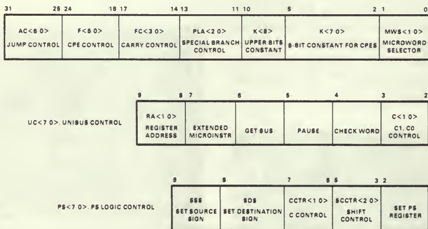
Figure 4. Microinstruction format.
