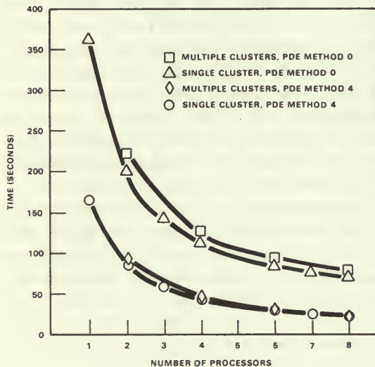
Figure 22. Single- and multiple-cluster execution time.
