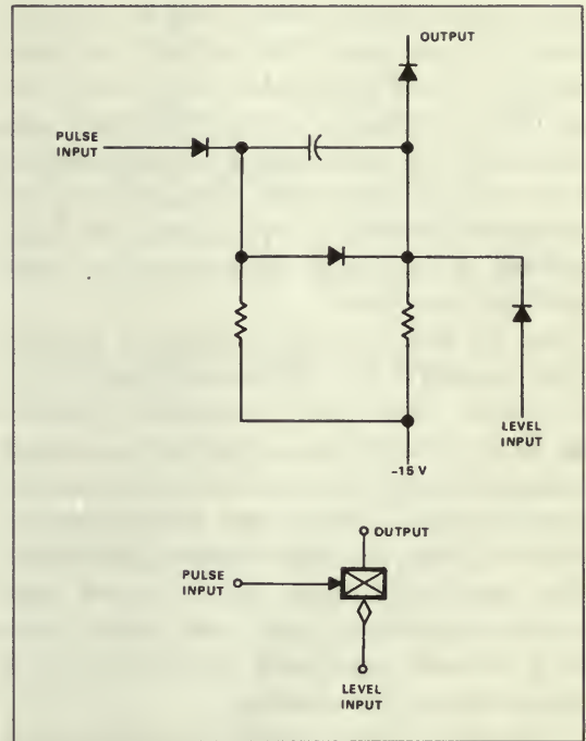
Figure 18. D-C-D gate.
