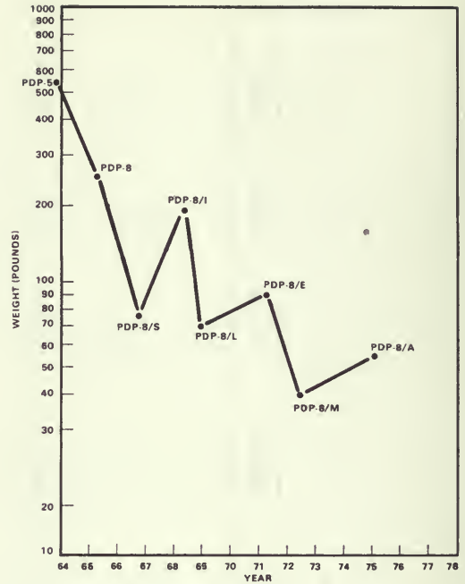
(b) Weight versus time.
