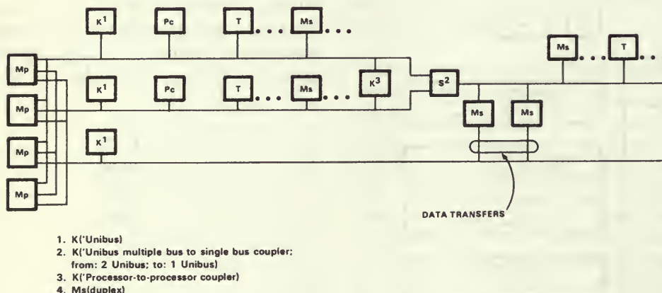
Figure 8. Dual Pc multiprocessor system PMS diagram.
