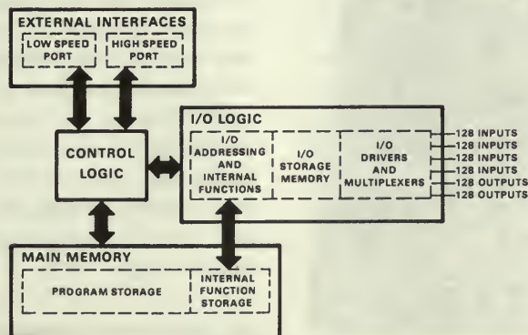
Figure 35. Block diagram of PDP-14/30.
