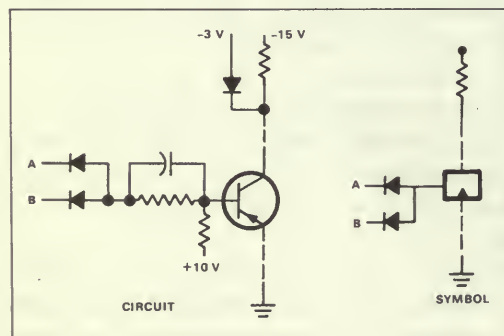
Figure 8. OR gate for negative signals.
