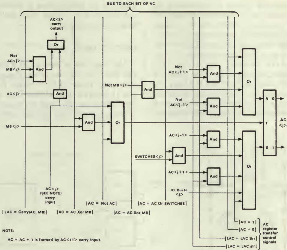
Figure 8. PDP-8 AC&lt;j&gt; bit logic diagram.
