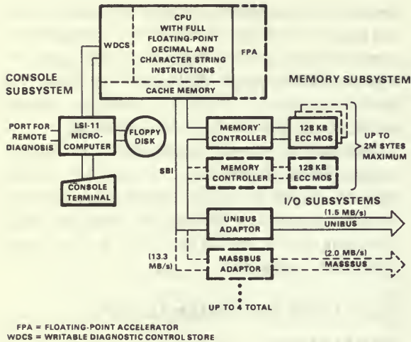
Figure 10. VAX-11/780 system.
