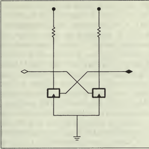
Figure 9. Primitive flip-flop.
