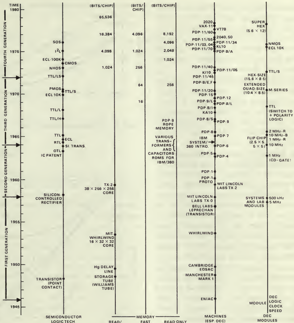
Figure 5. Logic and memory technology evolution timeline.
