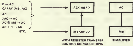
Figure 11. Register transfer representation of PDP-1 Accumulator (AC).
