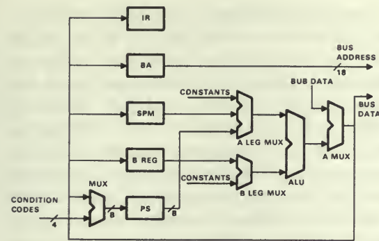
Figure 2. Archetypal medium-range PDP-11 data paths.
