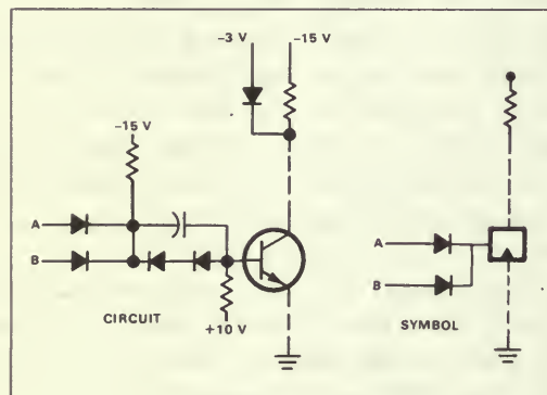
Figure 7. AND gate for negative signals.
