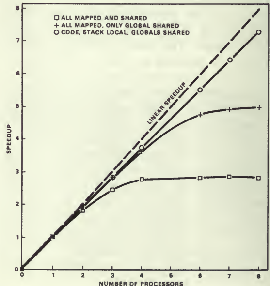
Figure 20. PDE speedup.
