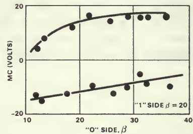
Figure 12. Beta margins.
