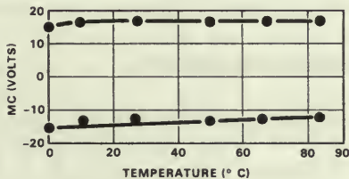
Figure 15. Temperature margins.
