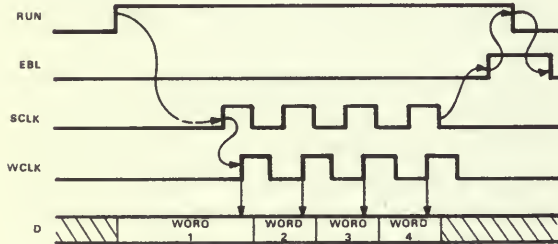
Figure 30. Timing of a Massbus Data Write.
