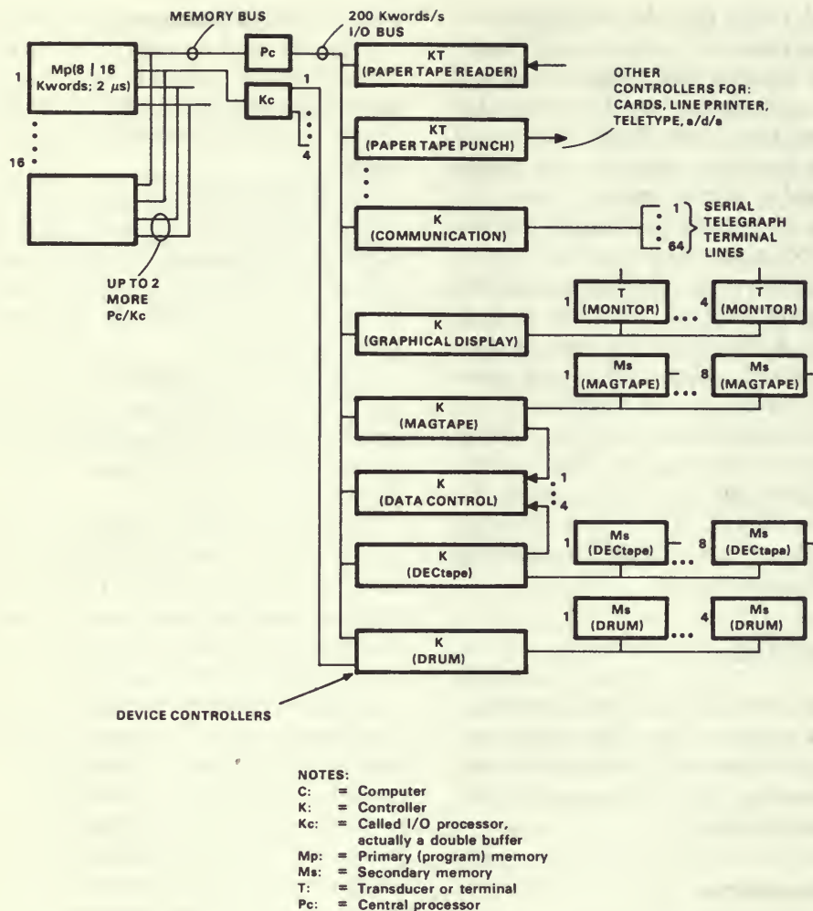
Figure 3. PMS diagram for PDP-6 system.
