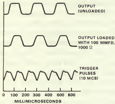
Figure 9. Flip-flop waveforms.
