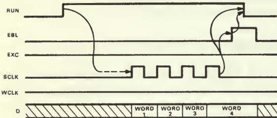
Figure 29. Timing of a Massbus Data Read.
