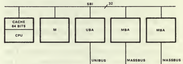
Figure 9. The VAX-11/780 organization, based on the SBI.
