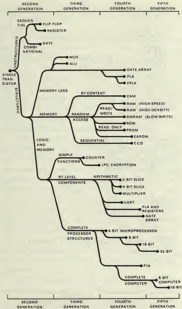
Figure 1. Family tree of digital integrated circuit functions.
