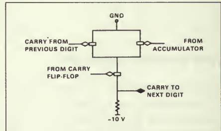
Figure 6. TX-2 carry circuits.
