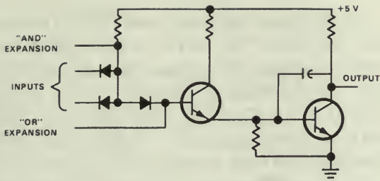
Figure 19. K-Series circuit.
