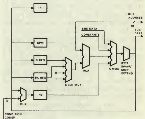
Figure 9. PDP-11/34 data paths.
