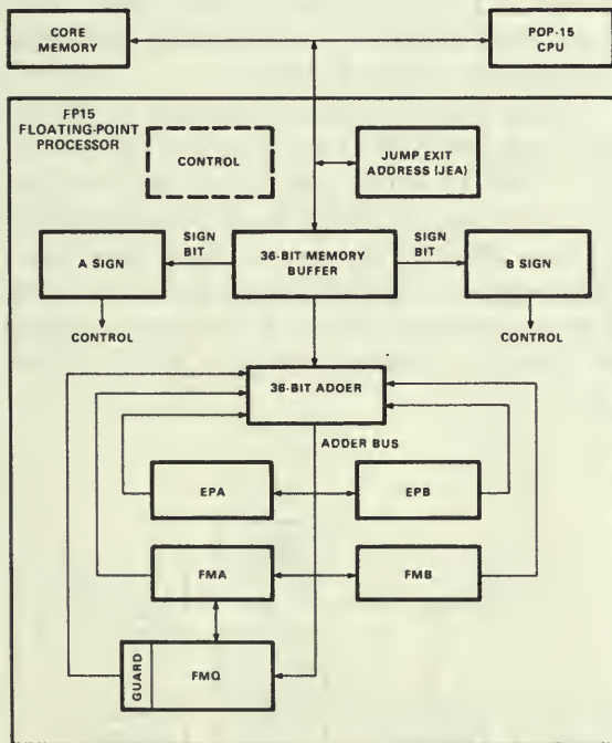
Figure 32. PDP-15 Floating-Point Processor register transfer diagram.
