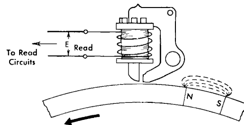
Figure II-55. Magnetic Reading Flux
