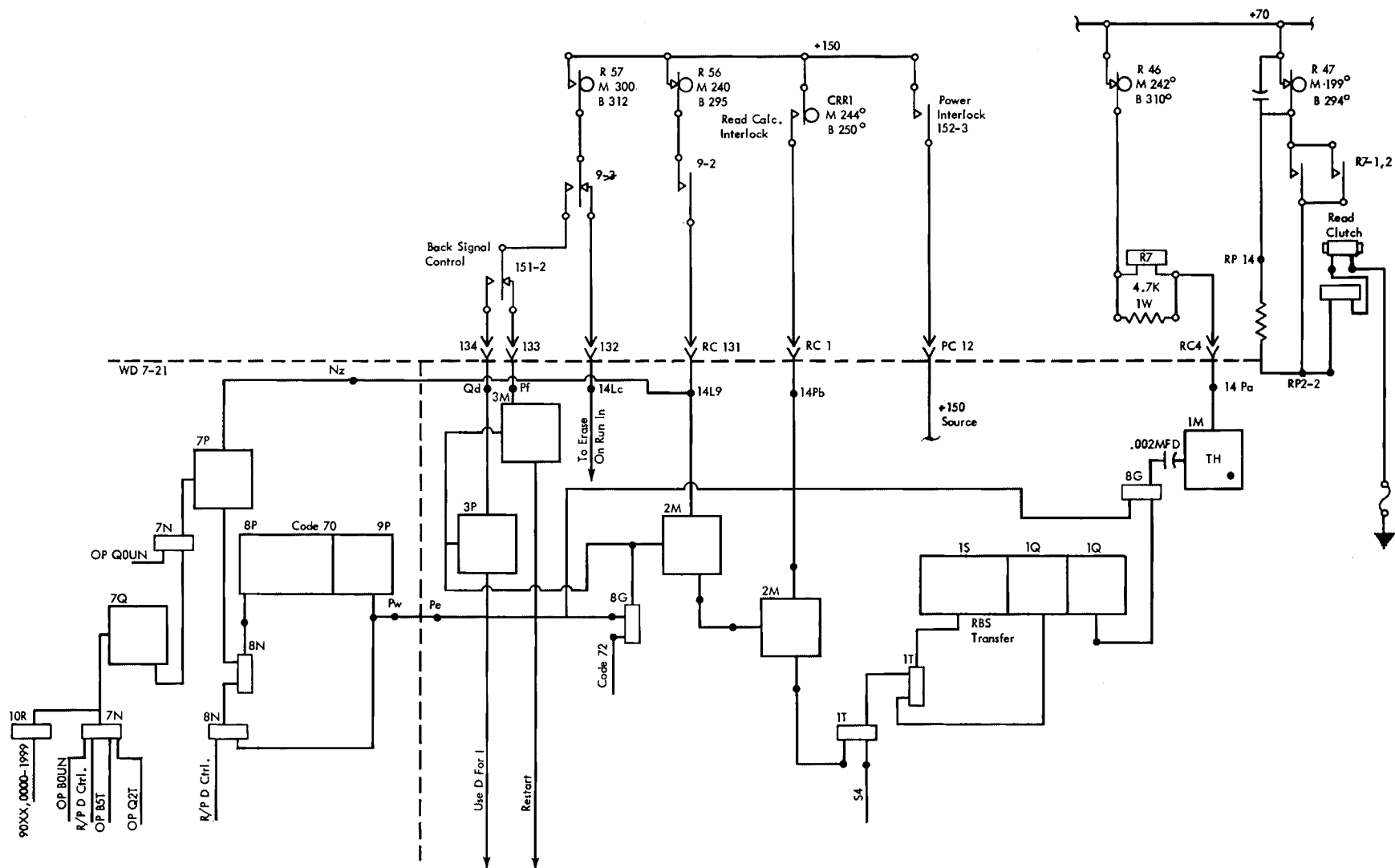
Figure VII-3. Read Feed Circuits
