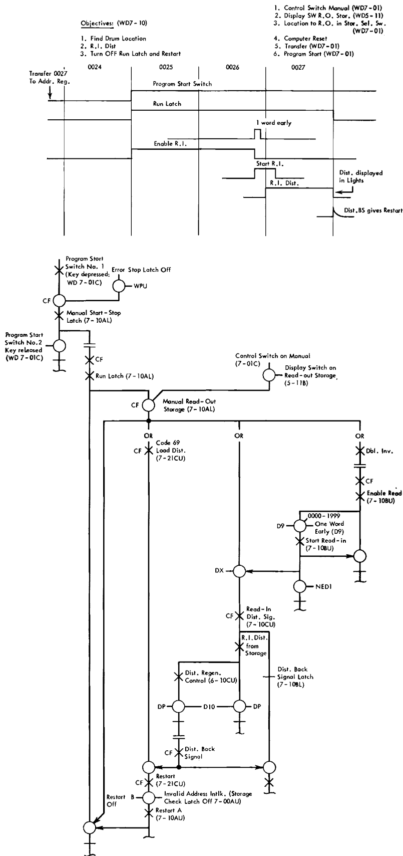
Figure VI-1. Manual Read-Out Storage
