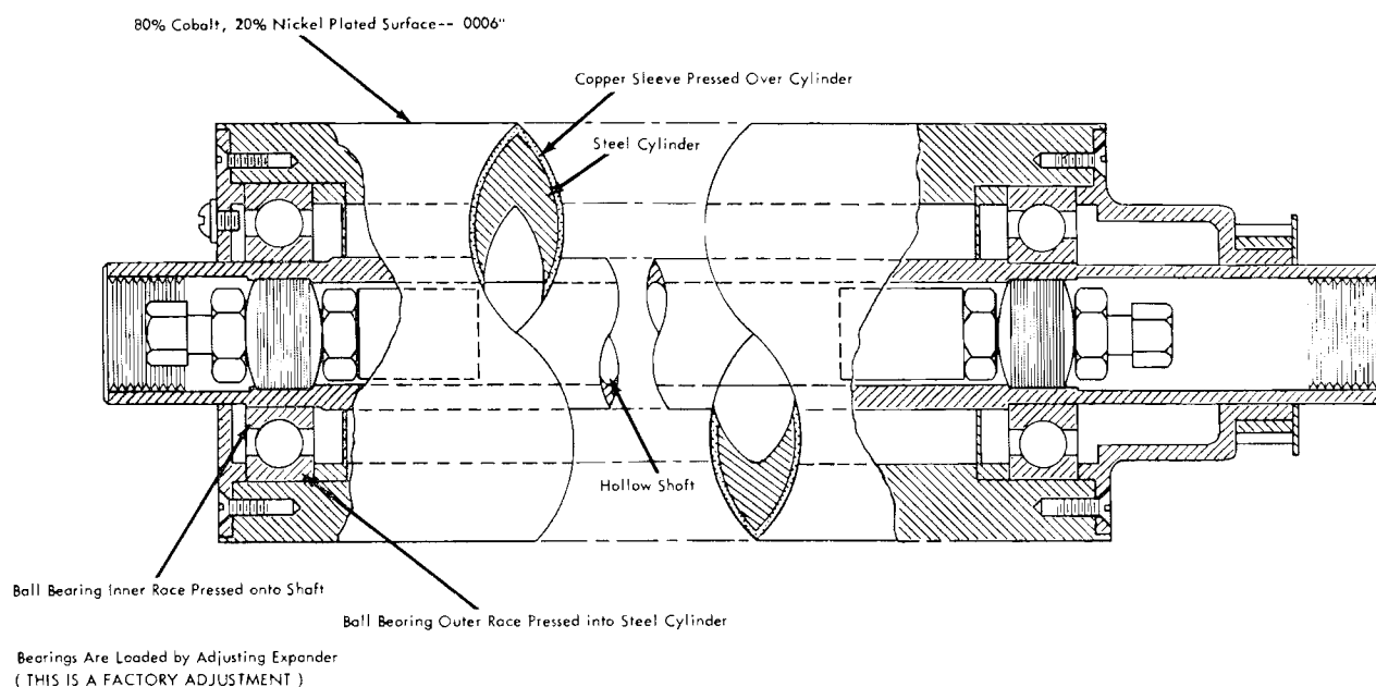
Figure II-58. Hollow Shaft Drum
