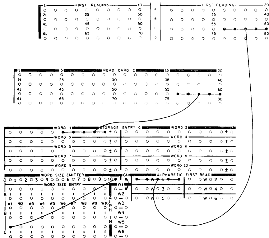
Figure VIII-1. Alphabetic Read-In Wiring
