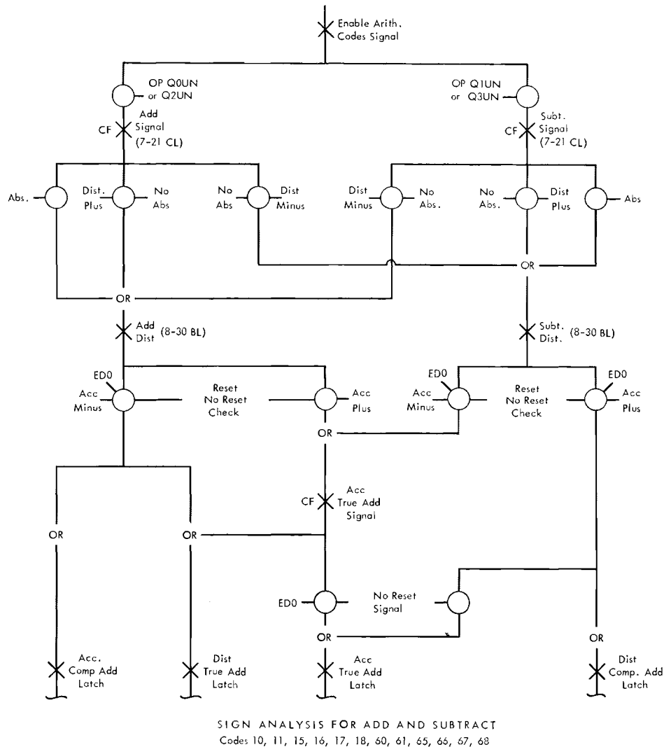
Figure V-13. Sign Analysis for Add and Subtract: Function Chart
