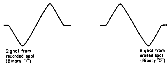
Figure II-56. Read Signals
