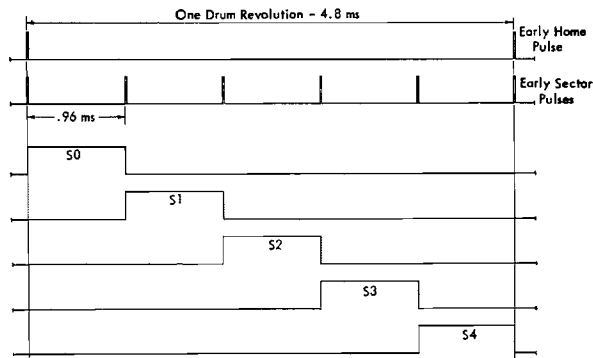
Figure II-35. Sector Gates
