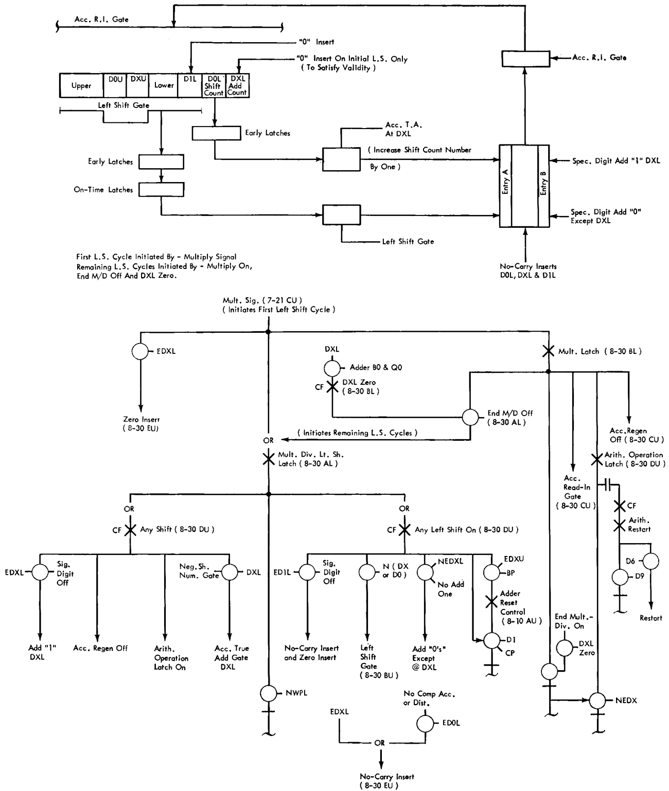
Figure V-38. Multiply Left Shift Cycle
