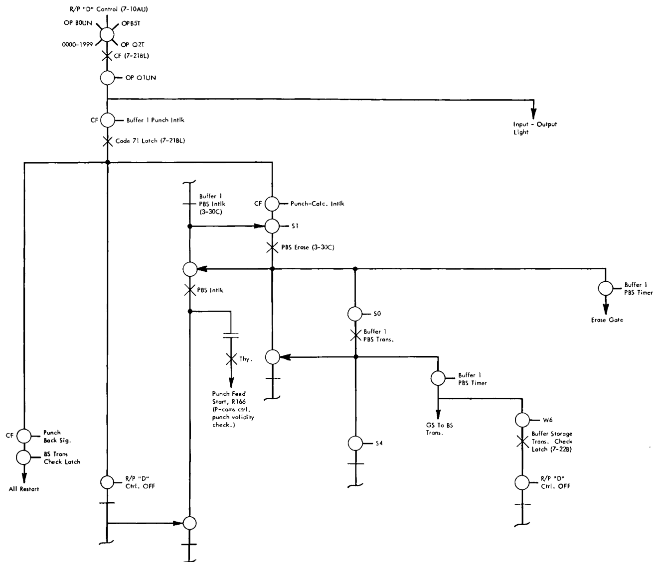
Figure VII-6. Punch—Code 71
