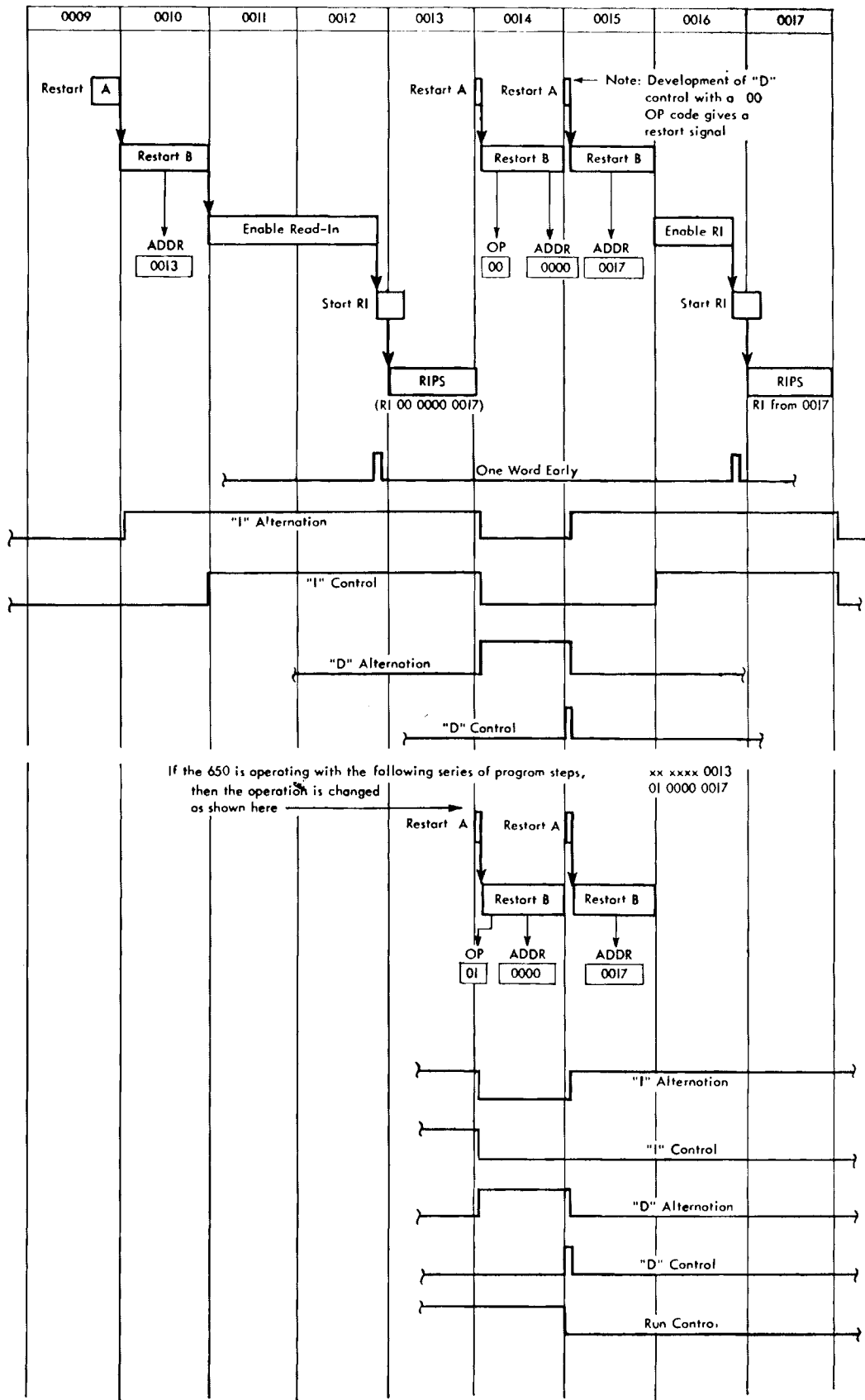
Figure V-14. Control Commutator Operation—Code 00 @ 01
