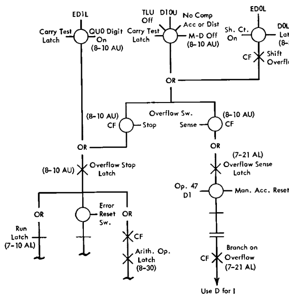
Figure III-5. Overflow Sense-Stop
