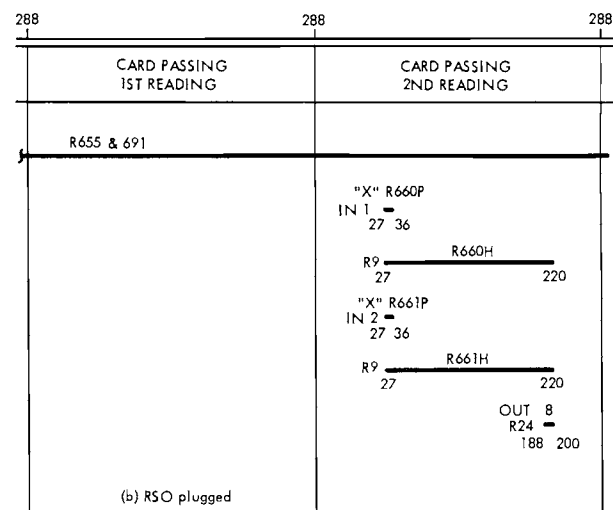
Figure X-9. Read Code Selector Operation
