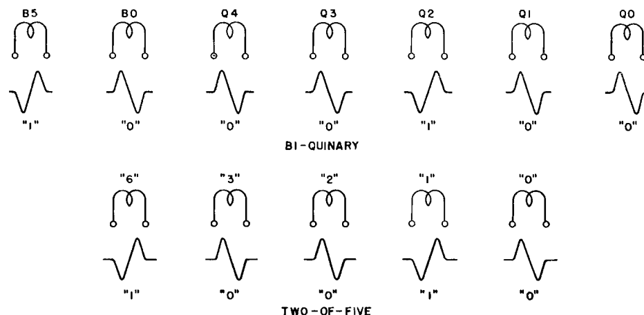
Figure II-57. Bi-Quinary and Two-of-Five Representations of Decimal 7
