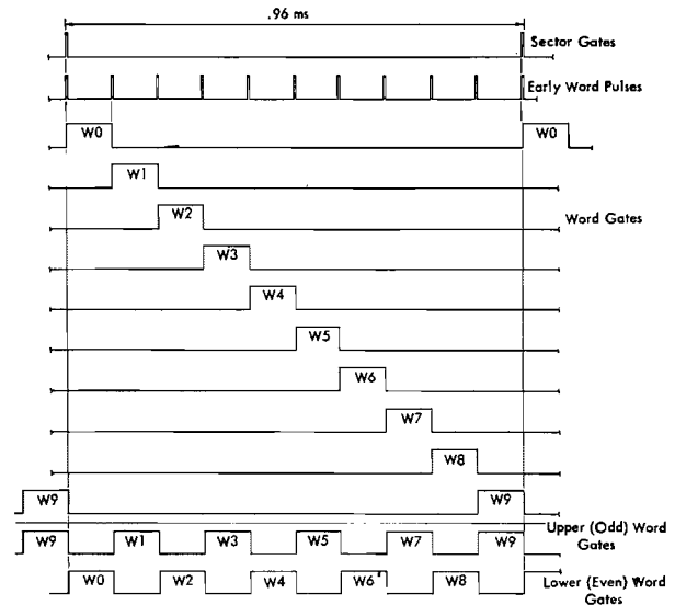
Figure II-36. Word Gates
