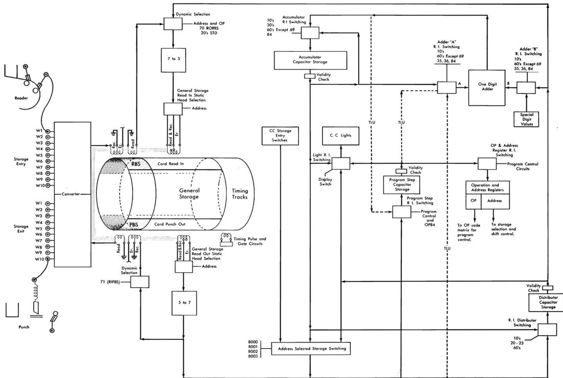
Figure I-11. 650 Logical Schematic
