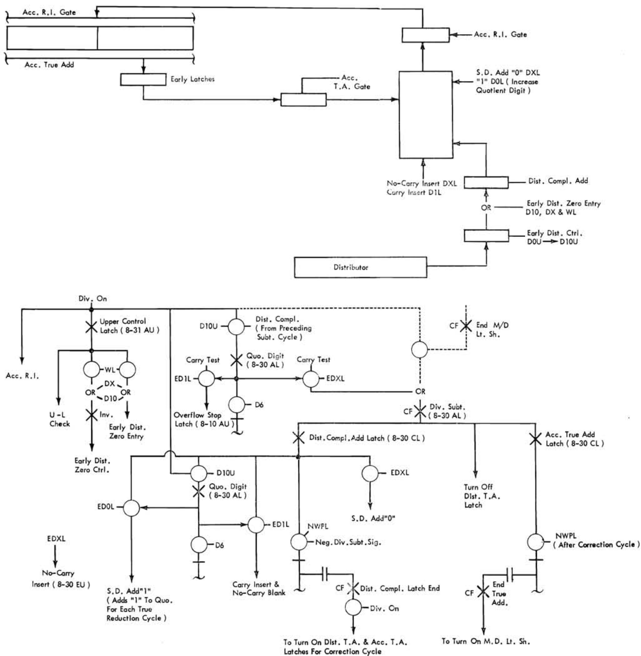
Figure V-50. Divide Subtract—Except First Cycle
