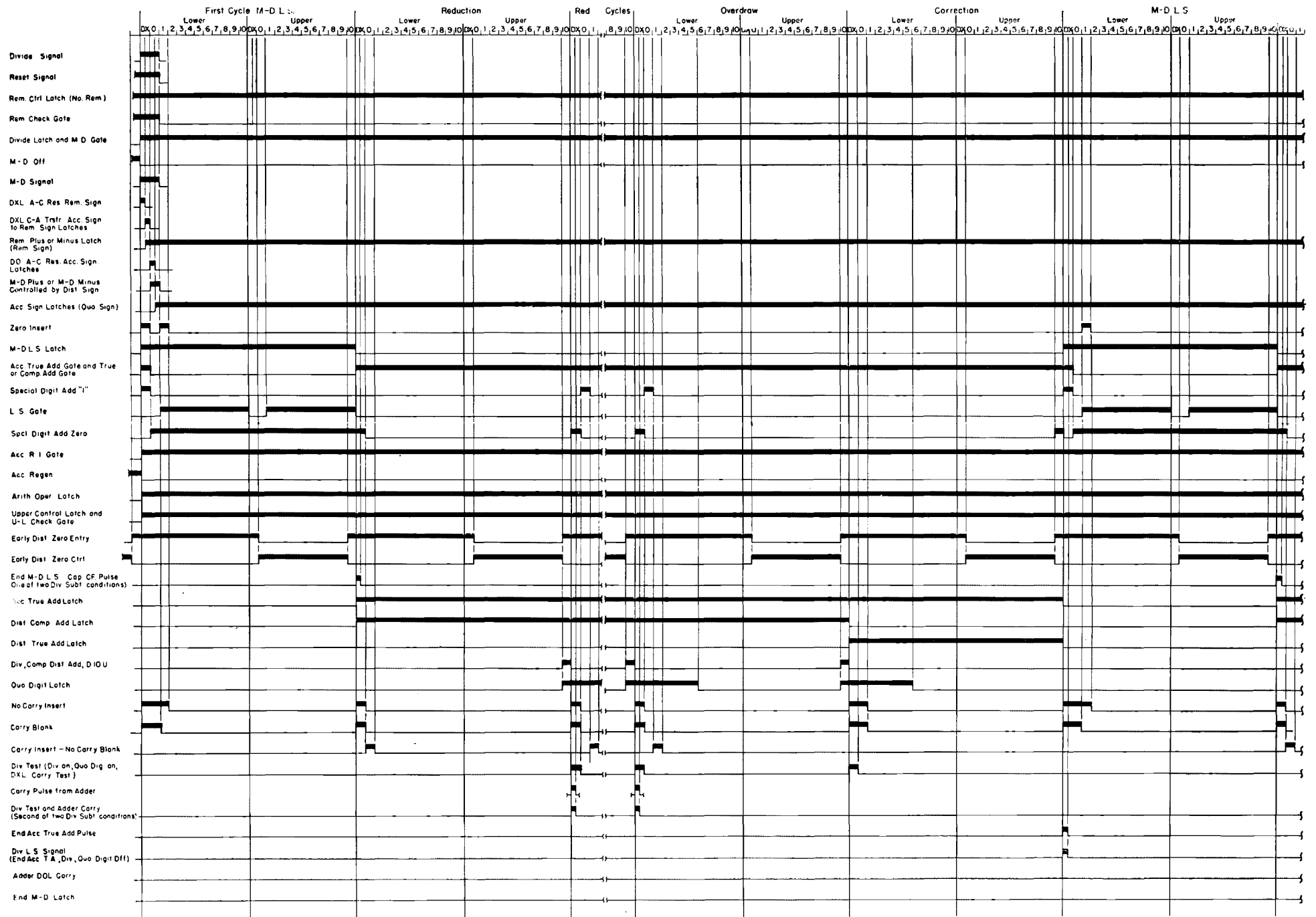
Figure V-52A. Divide Timing Chart
