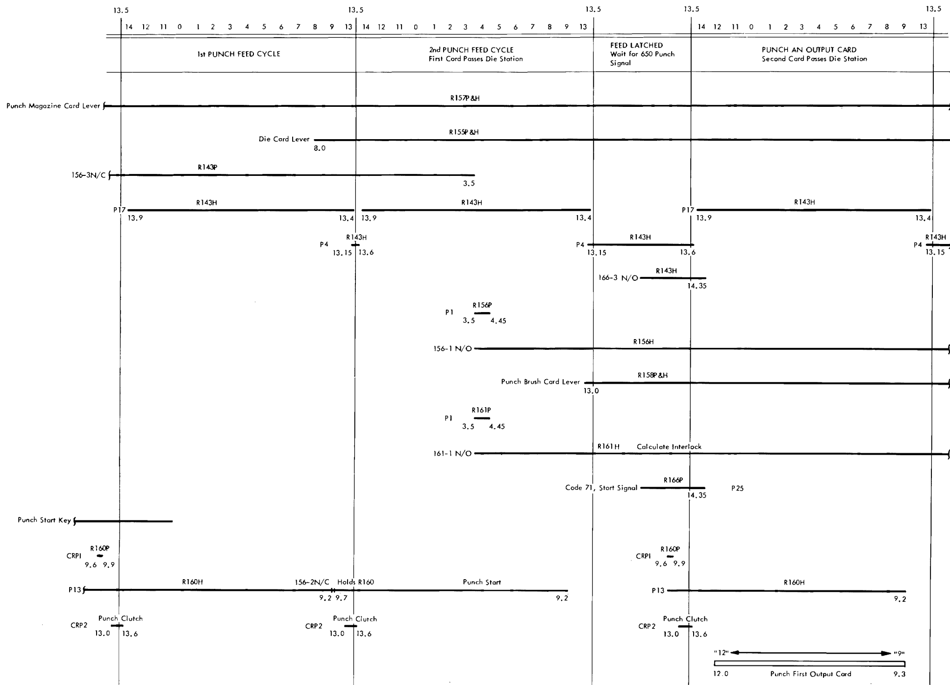
Figure X-11. 533 Punch-Feed Run-In Timing Chart
