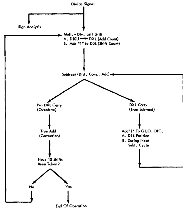
Figure V-45. Divide—Code 14
