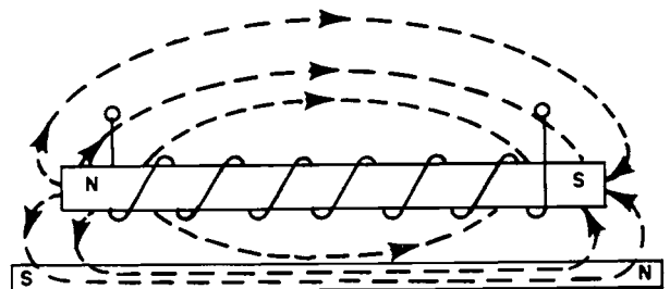
Figure II-52. Magnetic-Head Principles
