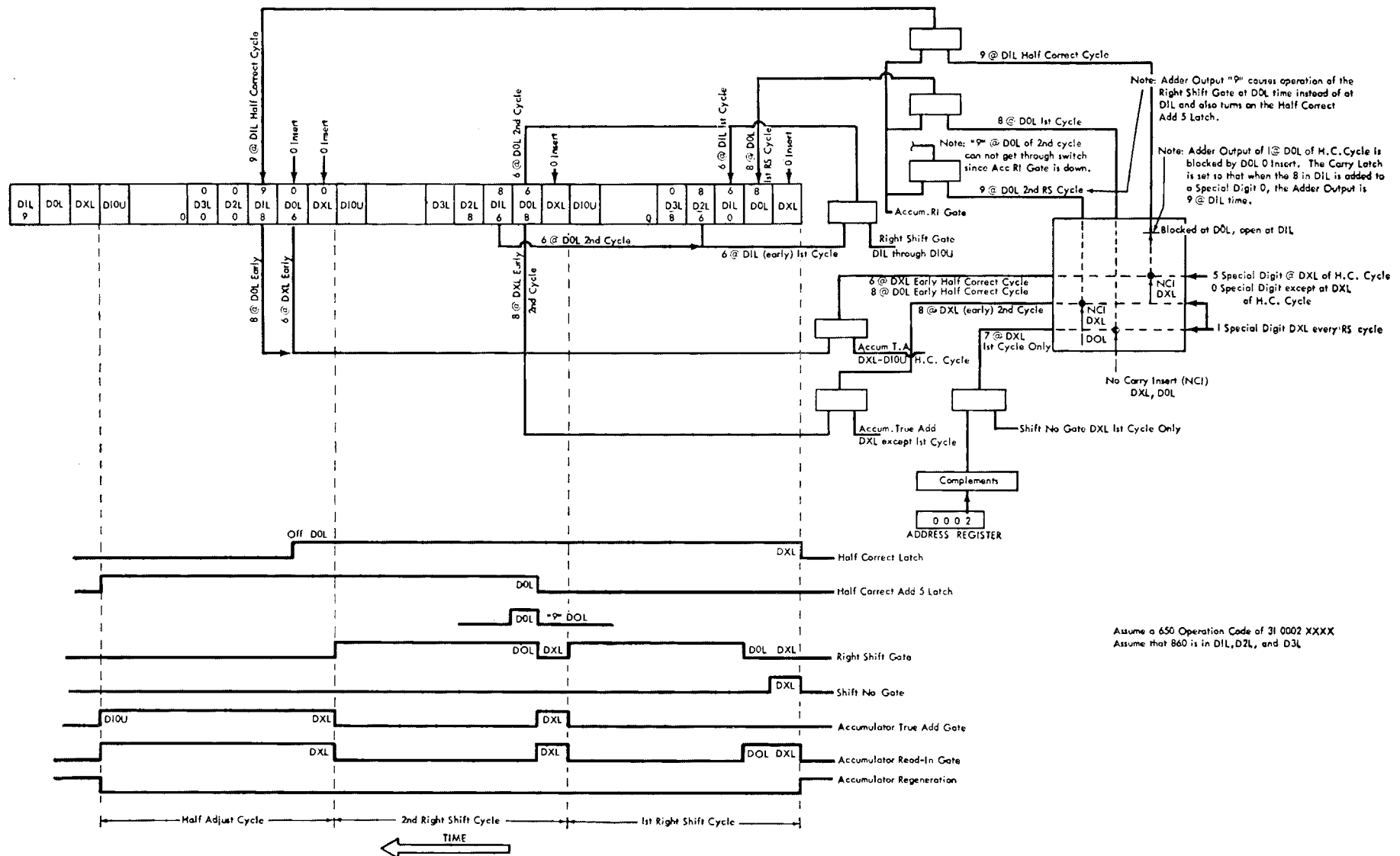
Figure V-23. Shift Right and Round: Block Diagram—Code 31
