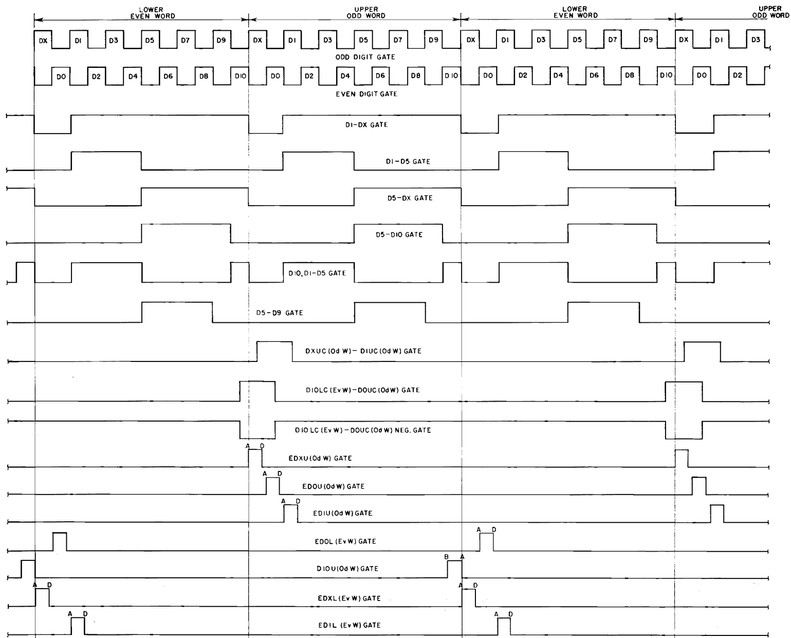
Figure II-38. Special Gates
