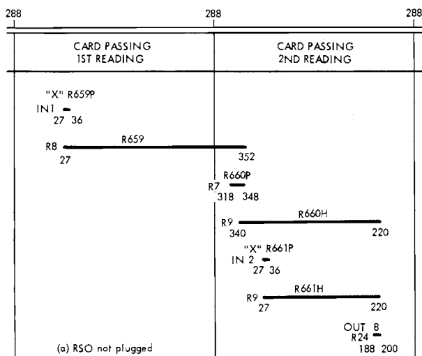
Figure X-9. Read Code Selector Operation
