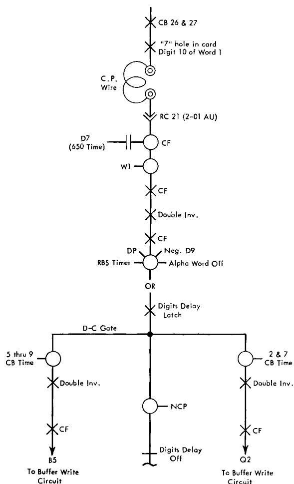
Figure VII-4. Scan a "7" Hole into Word 1, Digit 10 Position
