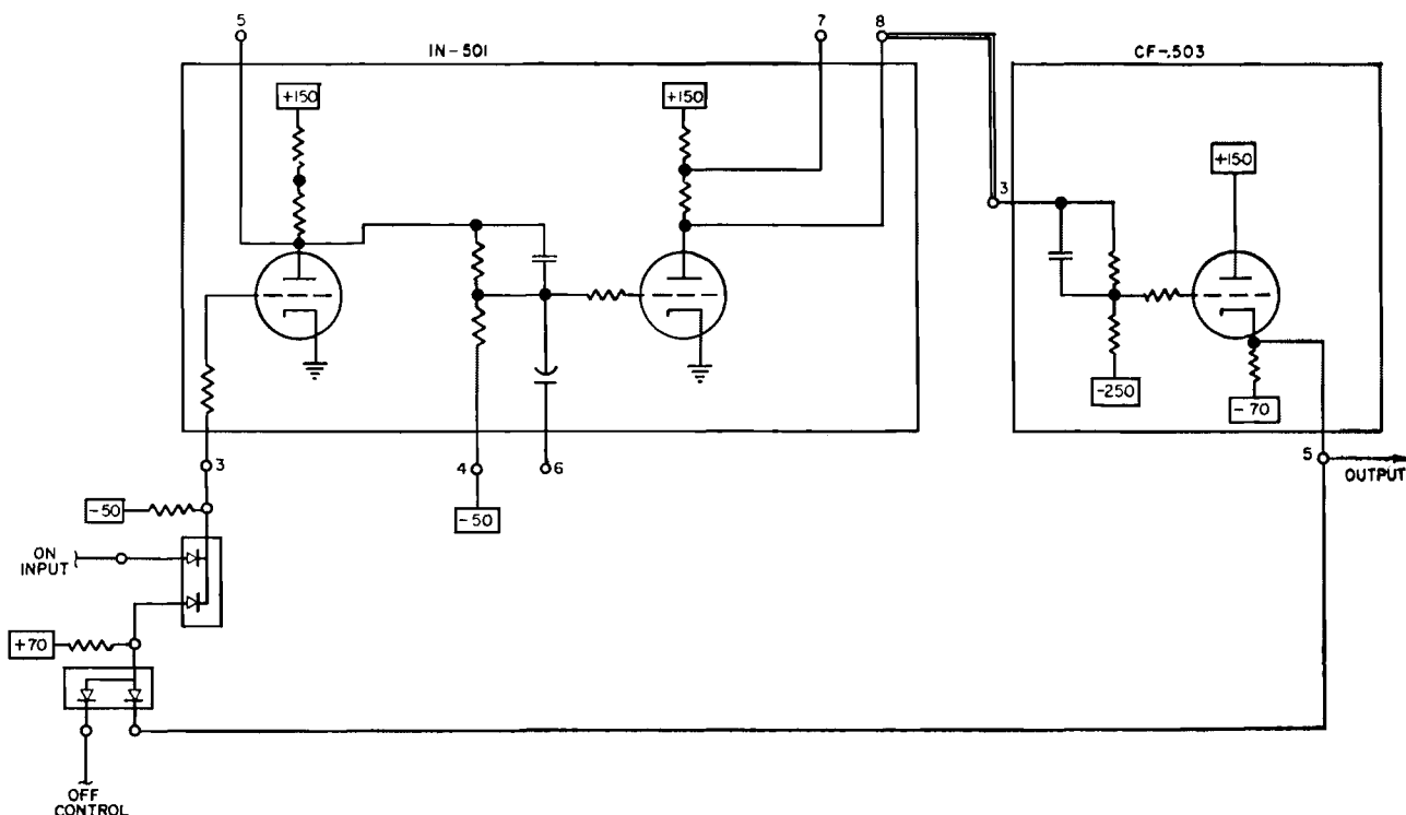
Figure II-19. Latch Circuit
