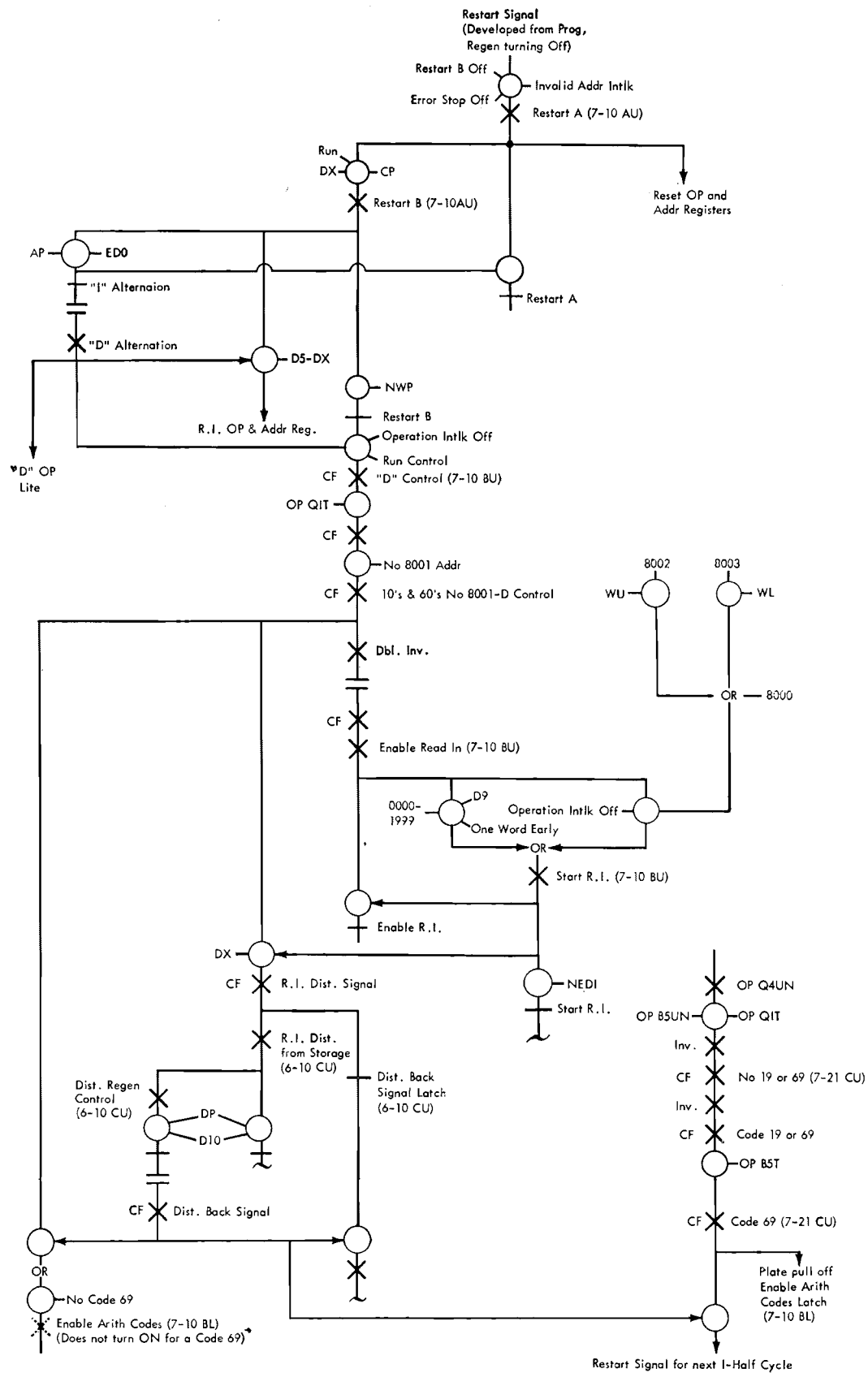
Figure V-5. D Half Cycle—Code 69
