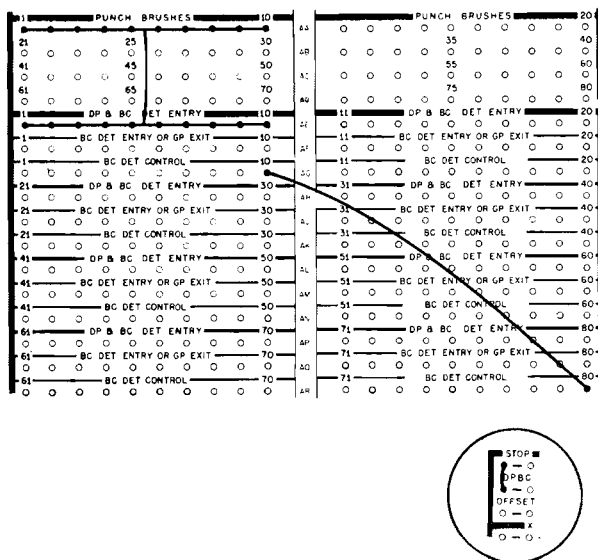
Figure X-6. Double-Punch and Blank-Column Detection Wiring
