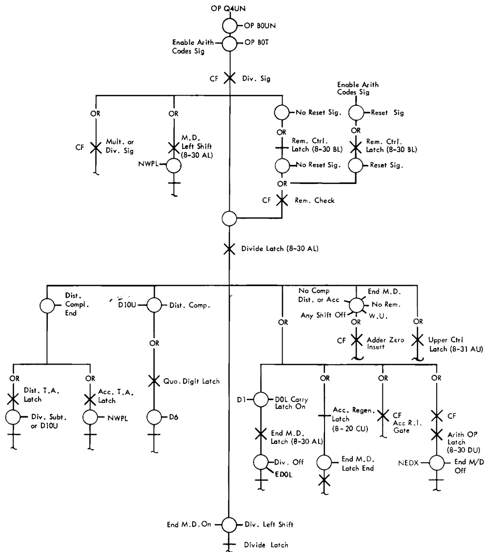
Figure V-46. Divide Controls
