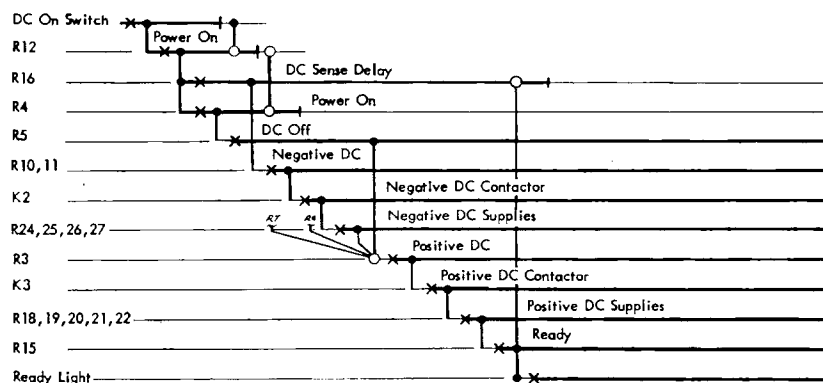
Figure IX-5. DC-On Sequence
