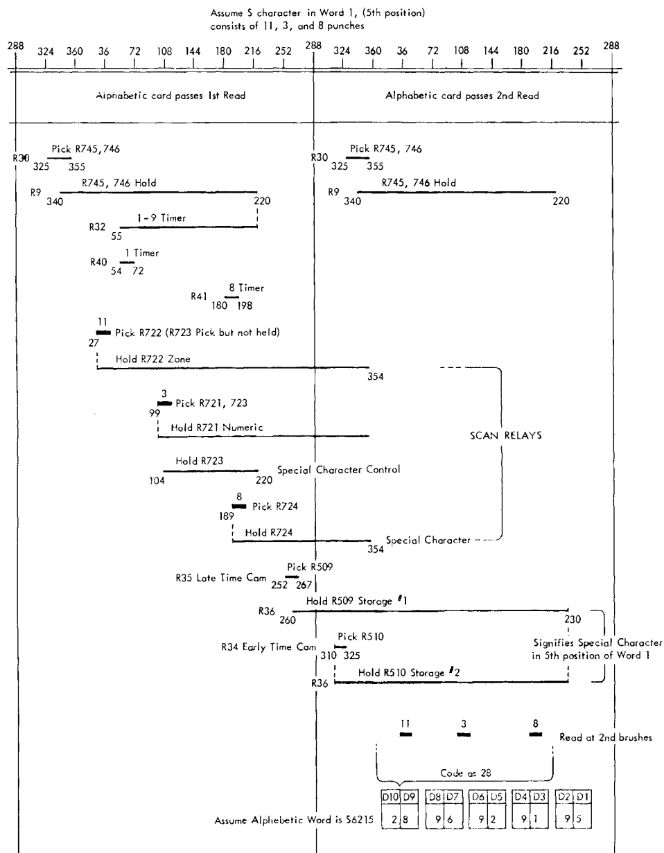
Figure VIII-6. Alphabetic Circuits Sequence Chart
