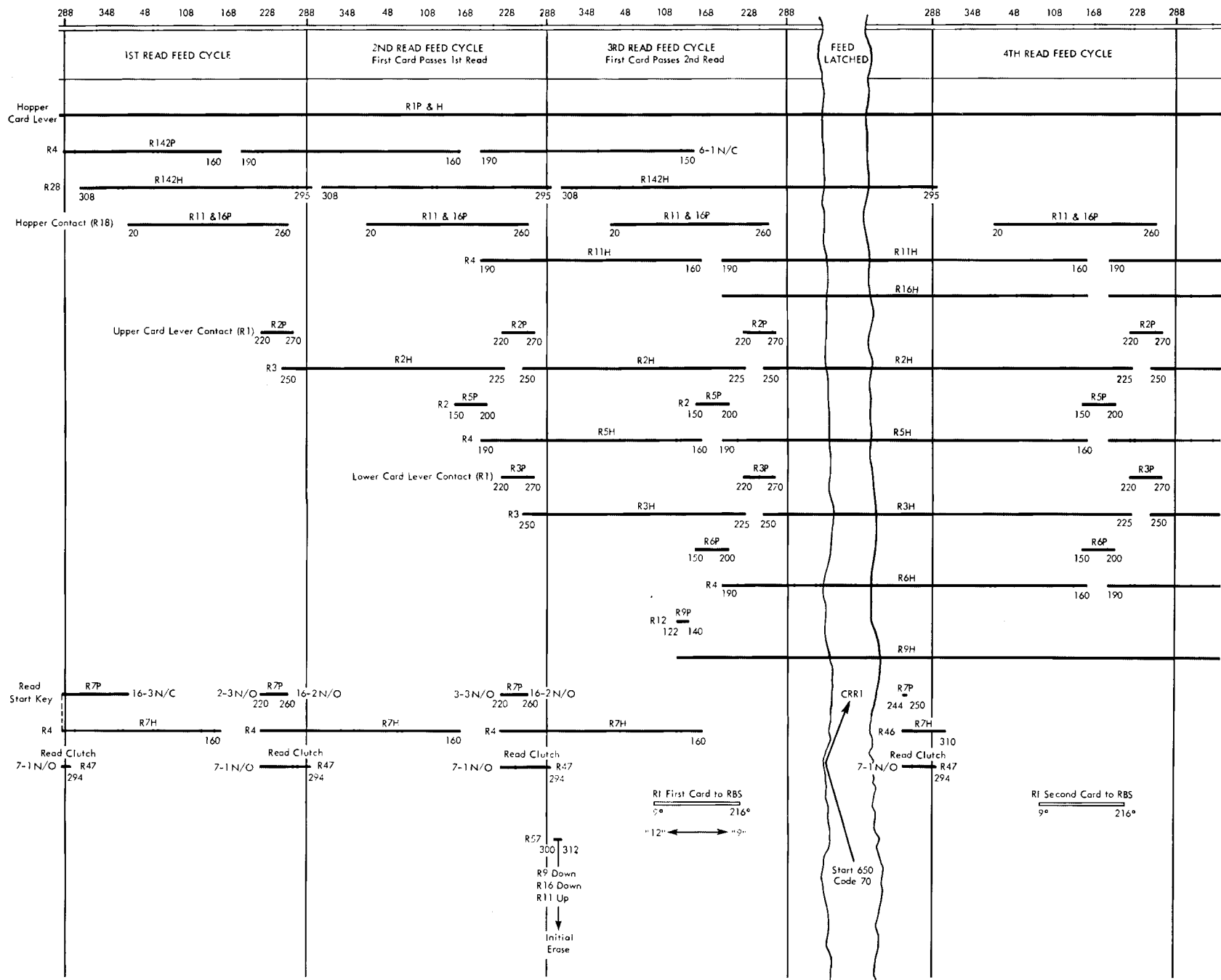
Figure X-10. 533 Read-Feed Run-In Timing Chart
