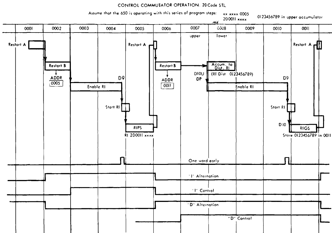
Figure V-17. Control Commutator Operation—Code 20
