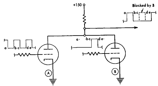
Figure II-9. Blocking Inverter
