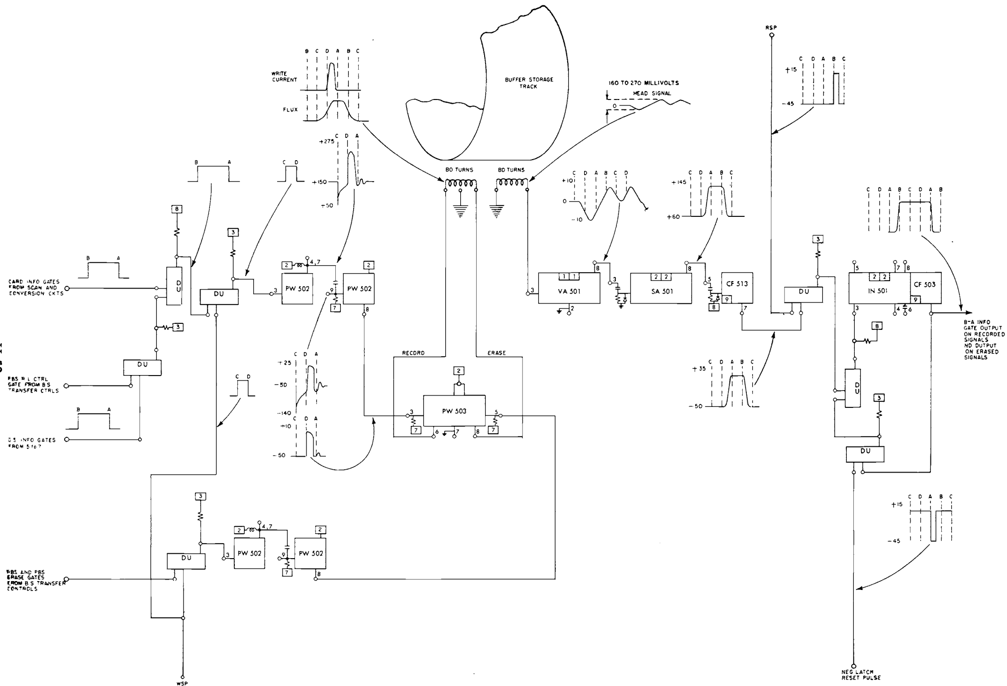
Figure II-63. Buffer Storage Head Connections and Read-Write Circuitry
