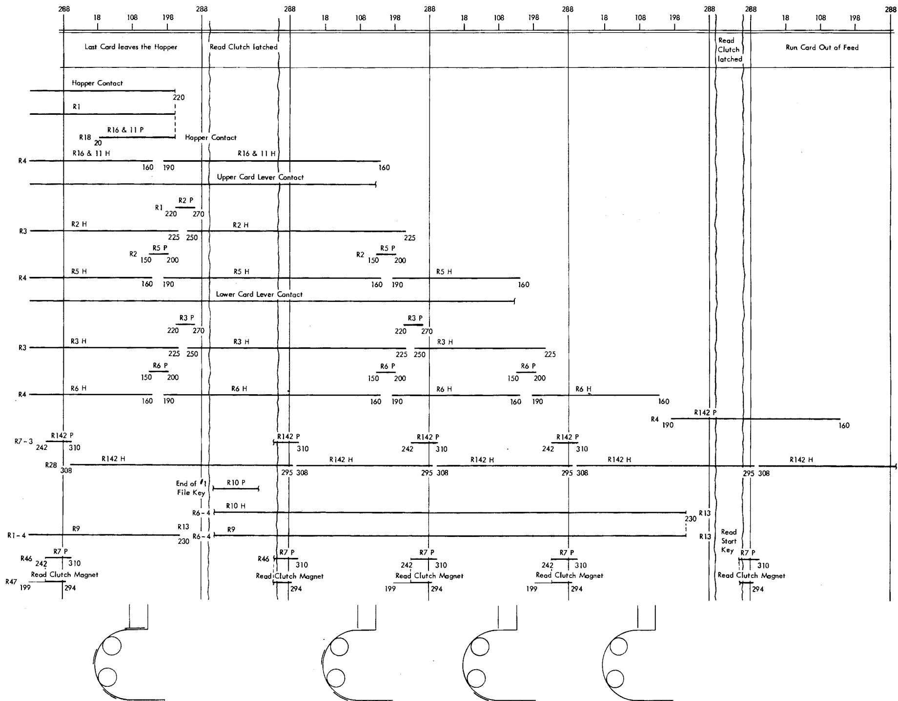
Figure X-13. 533 End-of-File Timing Chart
