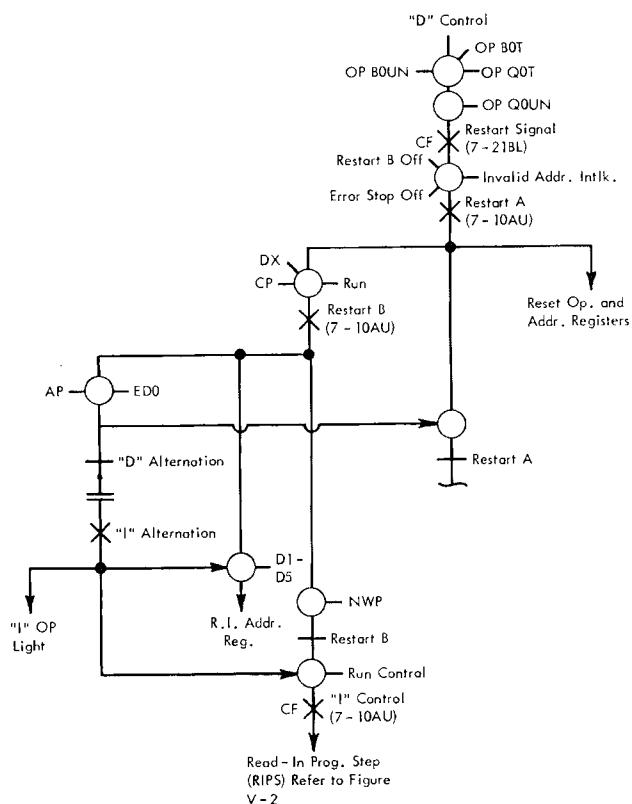
Figure V-15. No Operation—Code 00
