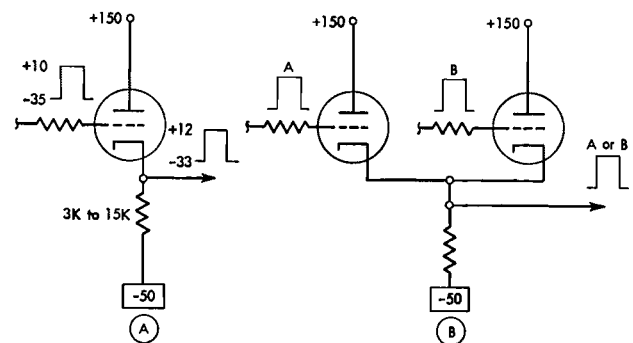
Figure II-10. Cathode Followers
