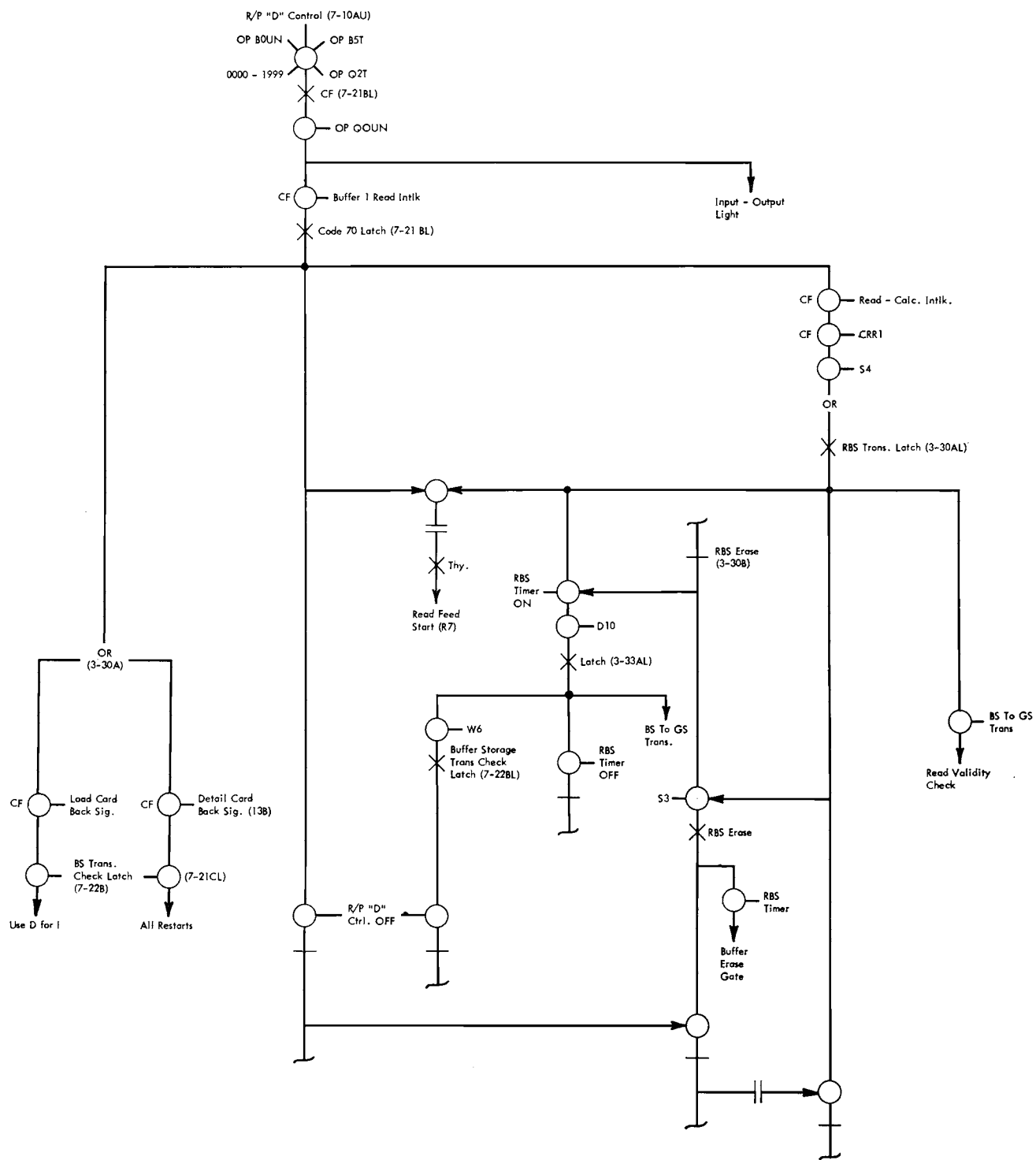
Figure VII-2. Read—Code 70
