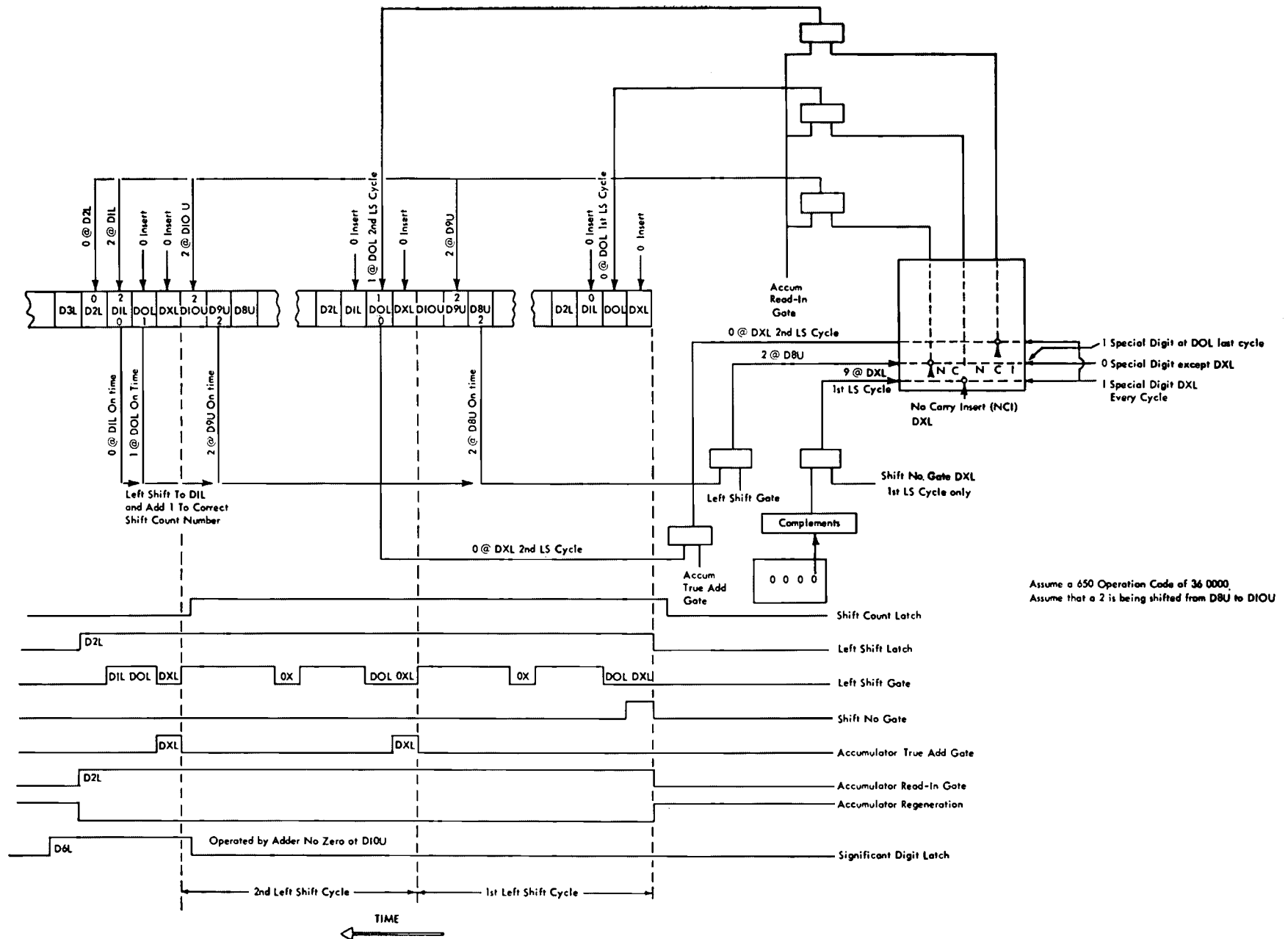
Figure V-28. Shift Left and Count: Block Diagram—Code 36
