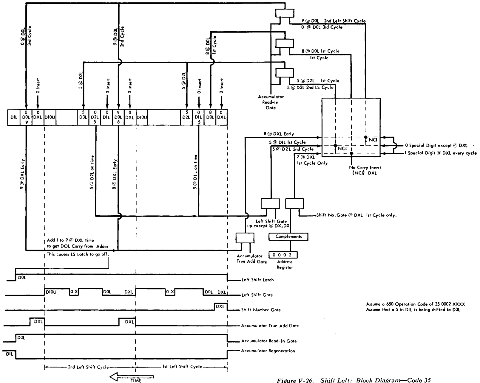
Figure V-26. Shift Left: Block Diagram—Code 35
