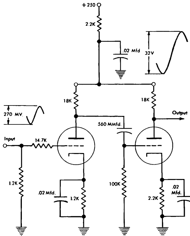
Figure II-23. Voltage Amplifier
