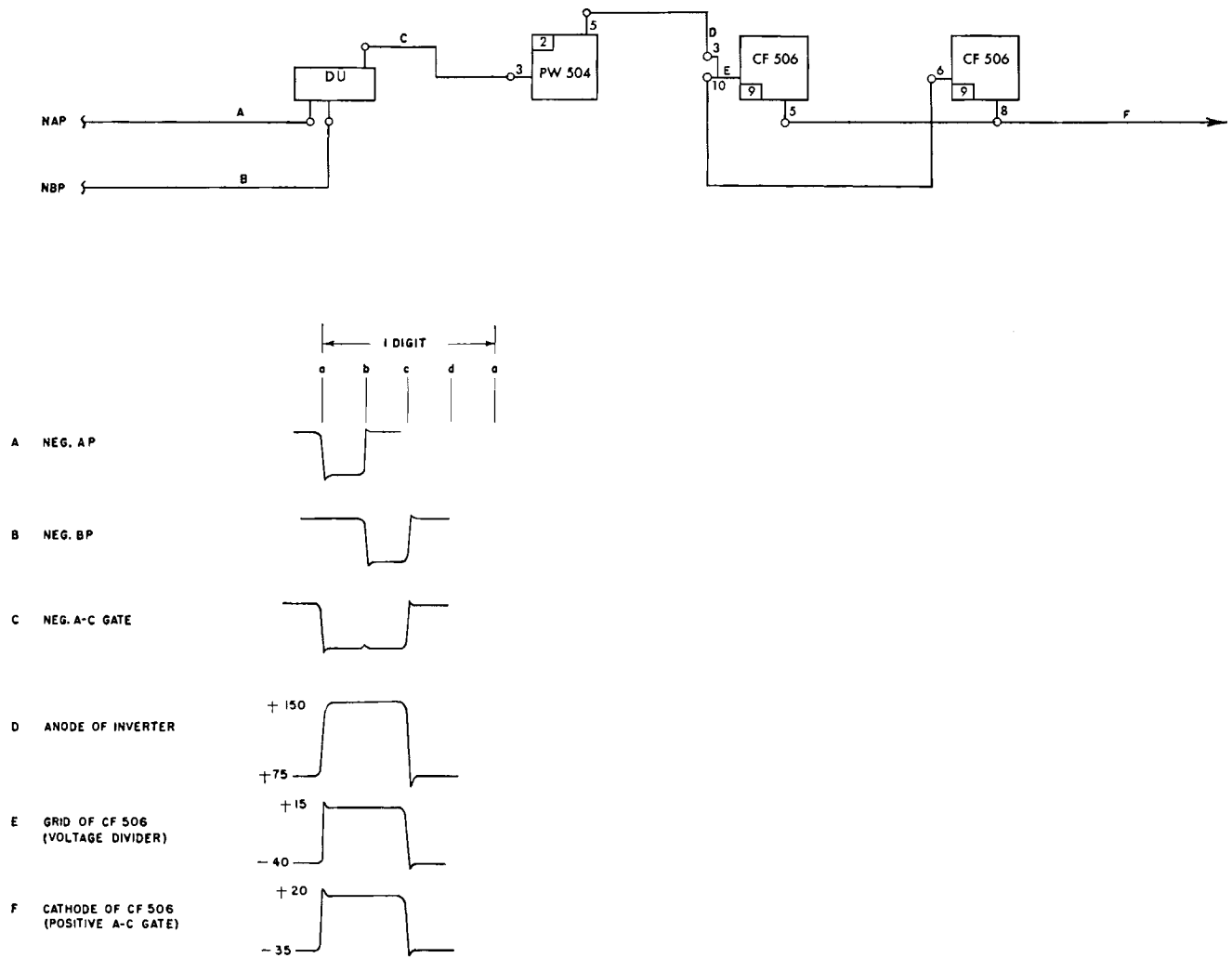
Figure II-48. Development of Special Timing Gate from Established Timing Pulses
