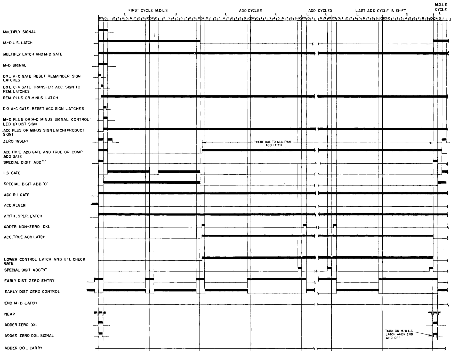
Figure V-41. Multiply Timing Chart
