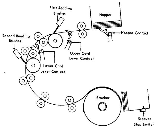
Figure X-1. 533 Read-Feed Schematic
