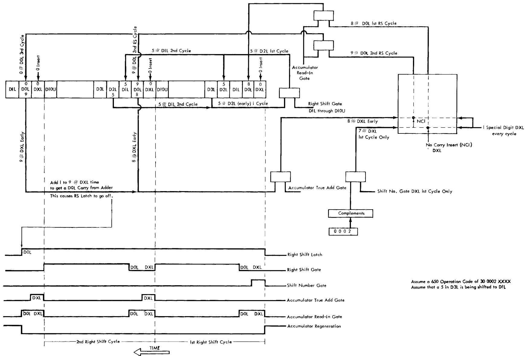
Figure V-21. Shift Right: Block Diagram—Code 30
