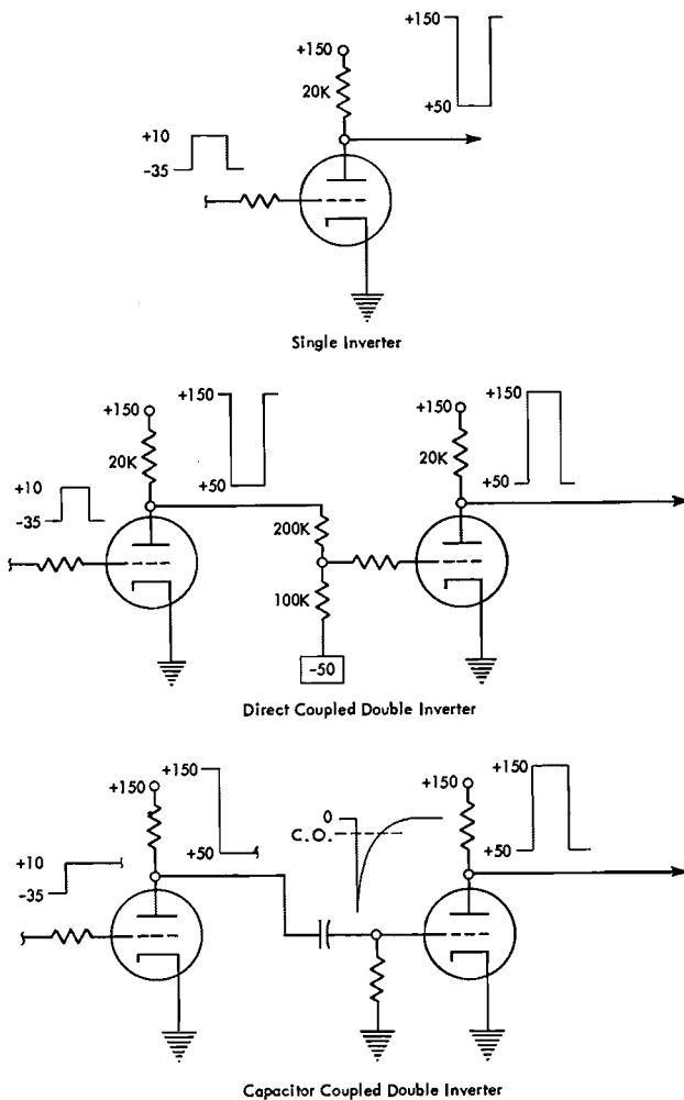
Figure II-7. Inverters
