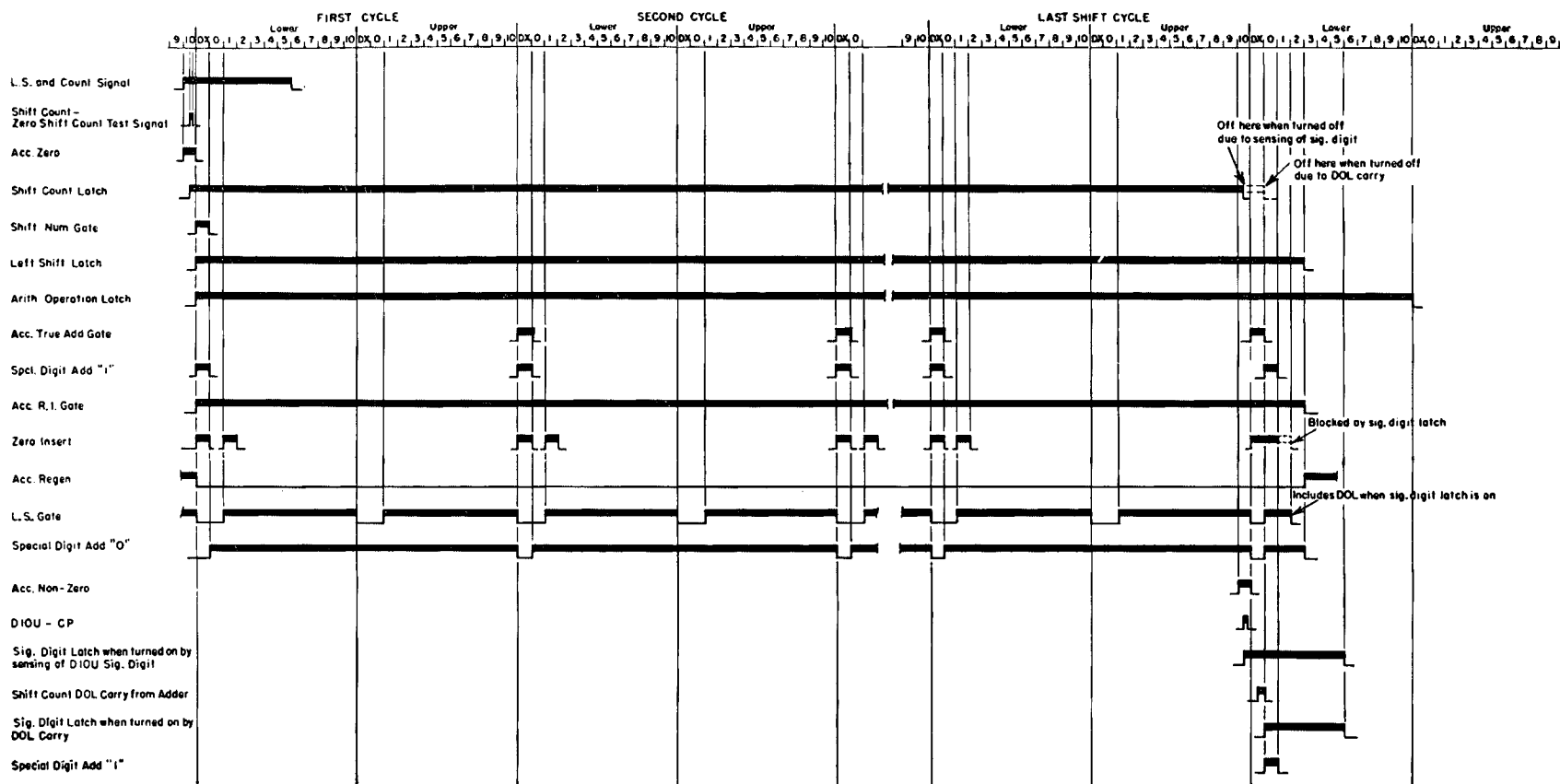
Figure V-29A. Shift Left and Count: Timing Chart, with Left Shift Cycles
