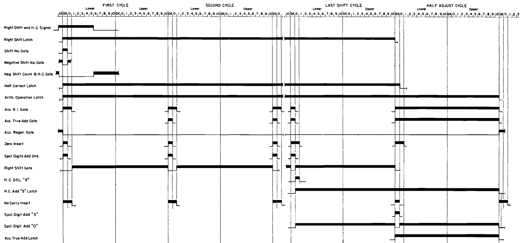
Figure V-25. Shift Right and Round: Timing Chart—Code 31
