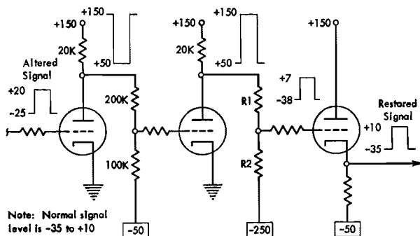
Figure II-8. Signal Level Restoration Using Double Inverter and Cathode Follower
