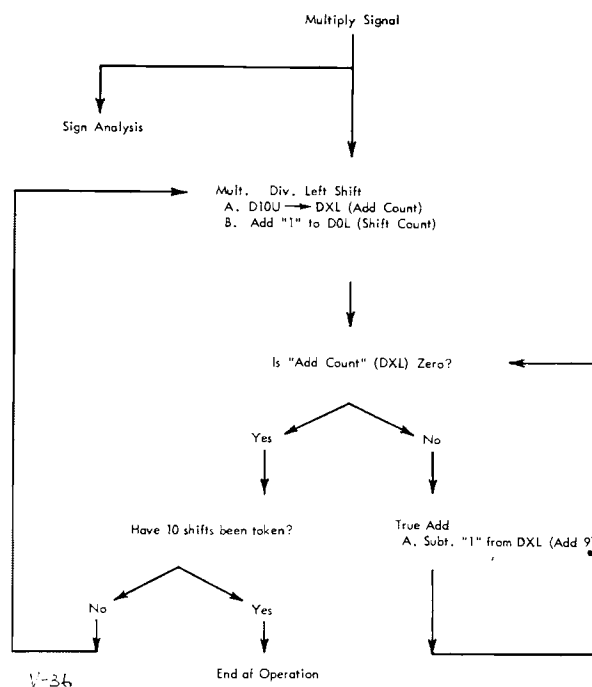
Figure V-36. Multiplication—Code 19
