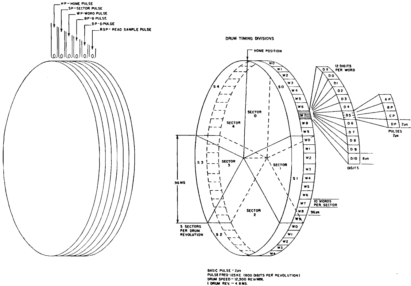
Figure I-8. Drum Timings
