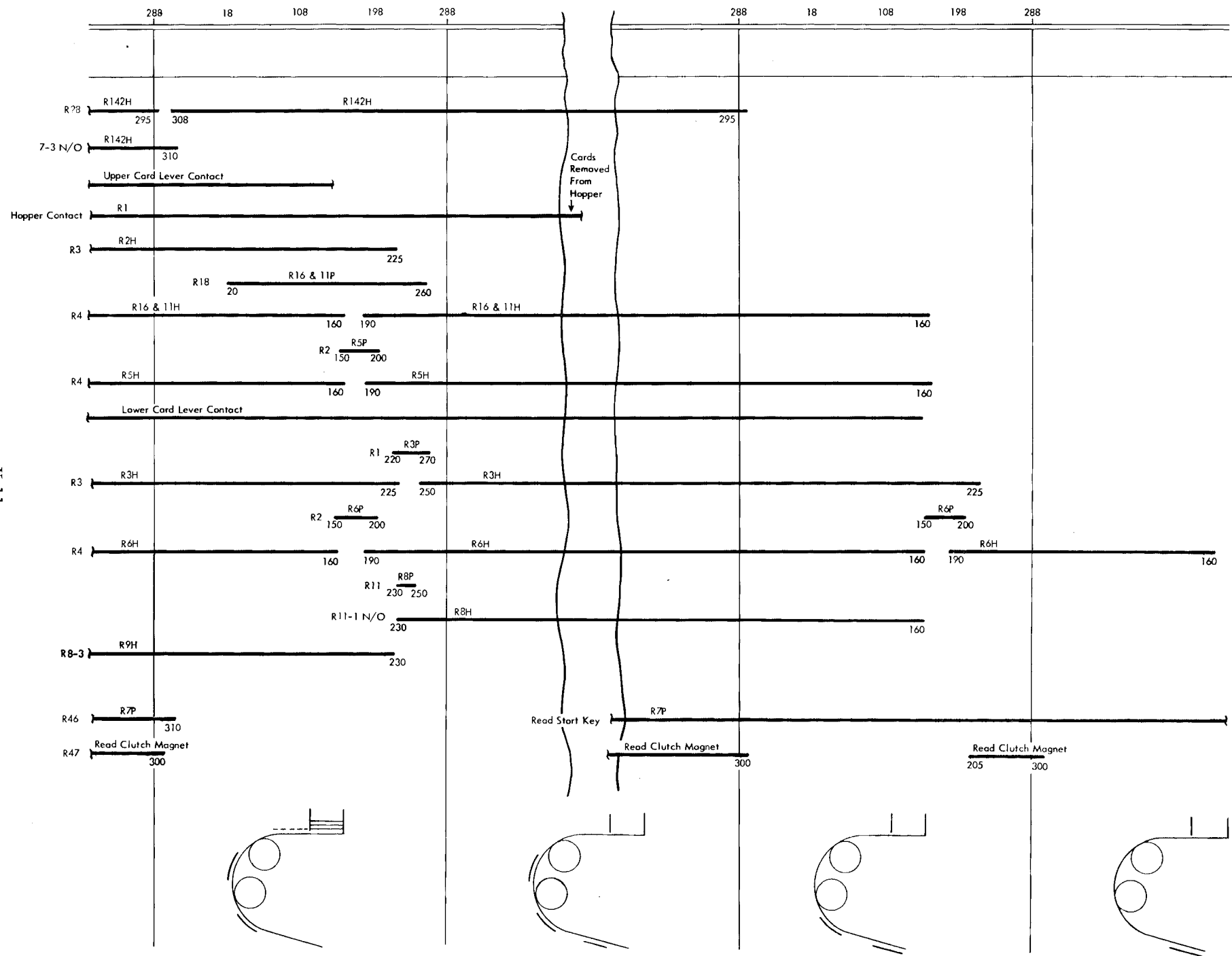
Figure X-12. 533 Card-Feed-Stop Timing Chart
