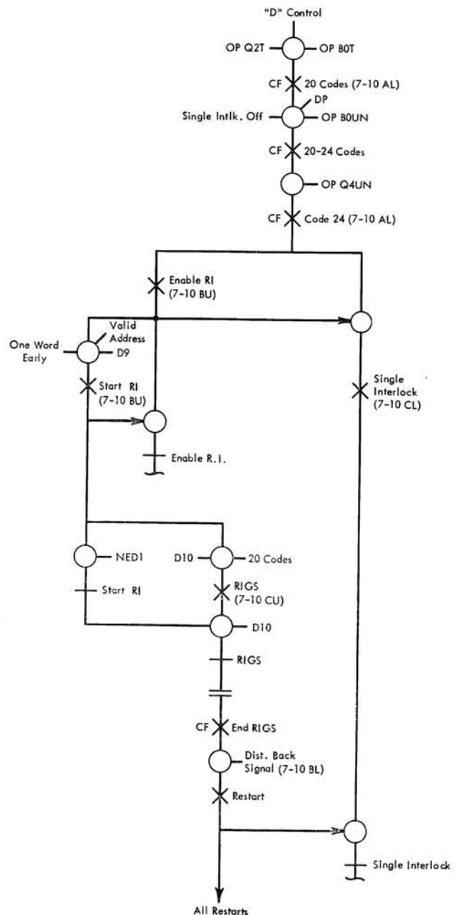
Figure V-19. Store Distributor—Code 24
