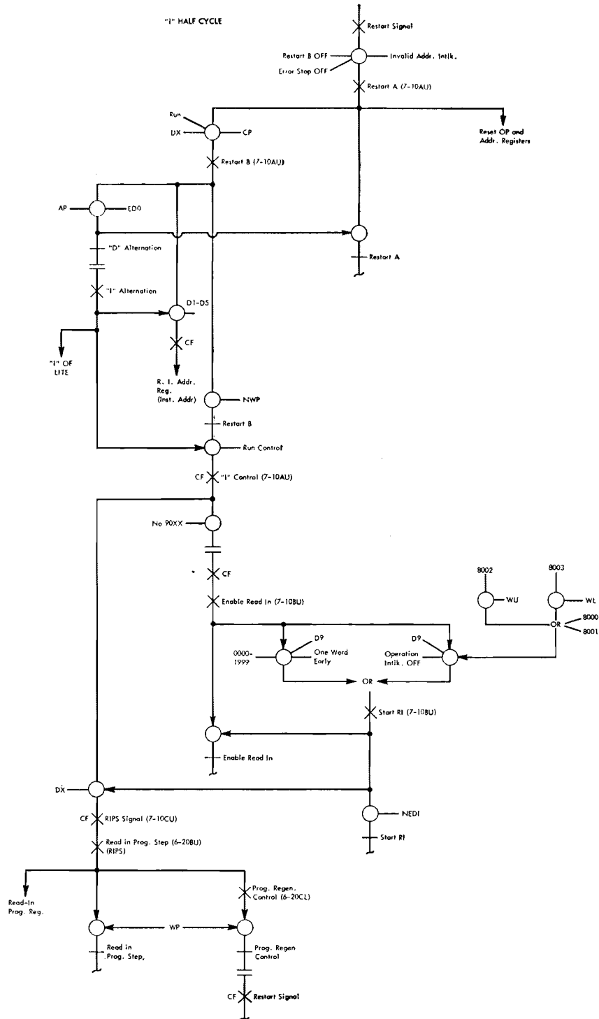
Figure V-2. 1 Half Cycle
