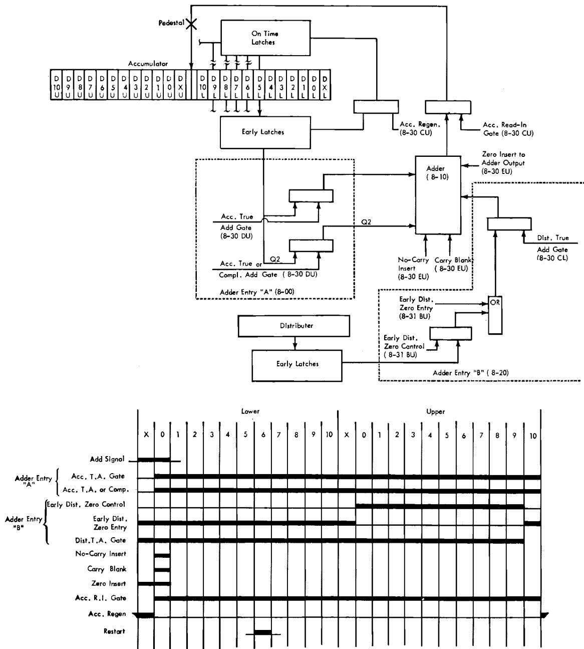
Figure V-6. Add Upper—Code 10
