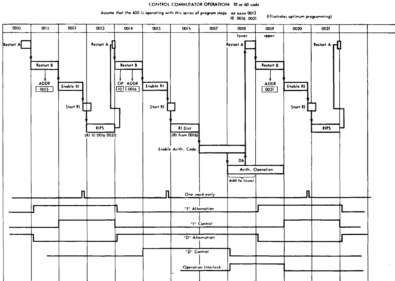
Figure V-3. Control Commutator Operation—Code 10-60's
