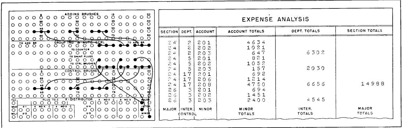
Plugging for Automatic Control
