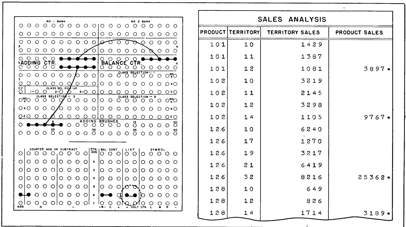
Wiring For Addition
