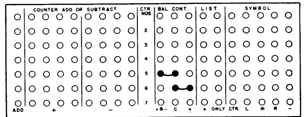
Wiring of Symbol Hubs
