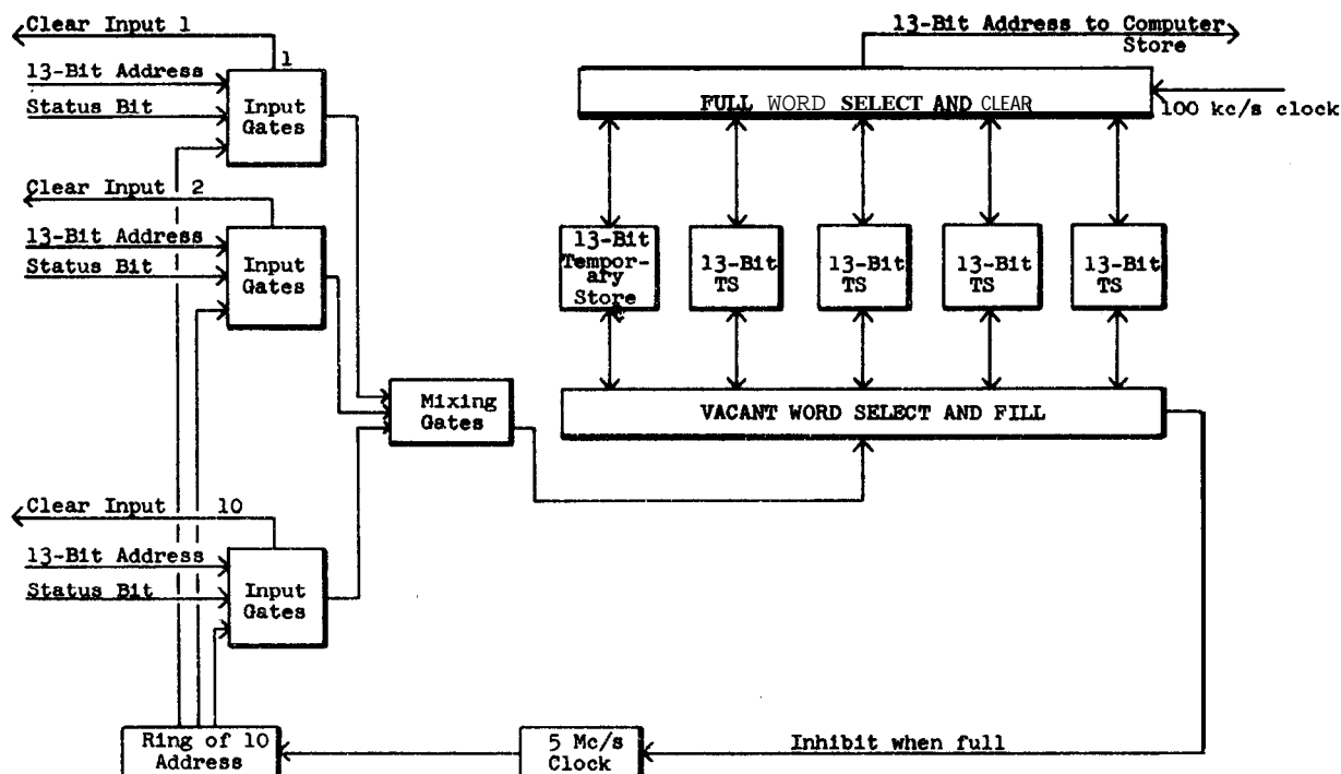
Fig. 5. Derandomizer logic.
