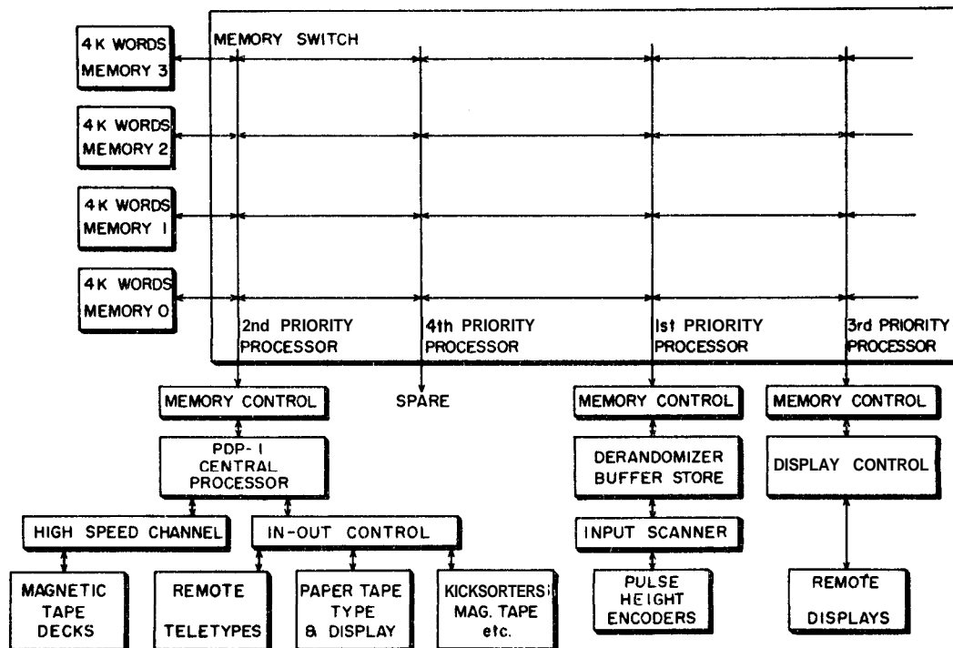
Fig. 4. Time-shared memory.
