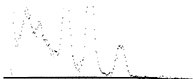
Fig. 2. \text{Cu}^{63} spectrum taken at 45^\circ .
