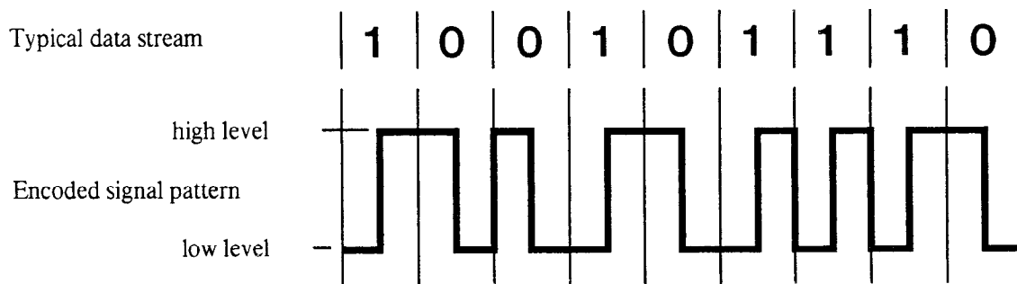
Figure 7-6: Manchester Encoding
