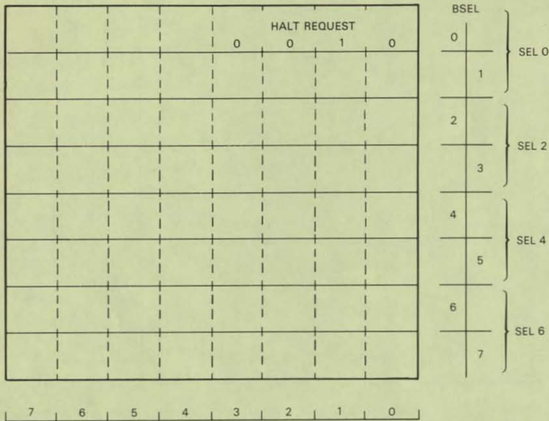
Figure 3-12 Halt Request Command Format
