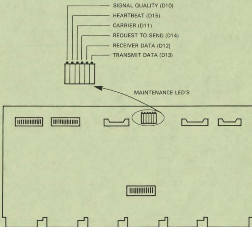
Figure 4-1 M8203 Maintenance LED Locations/Heartbeat Waveform
