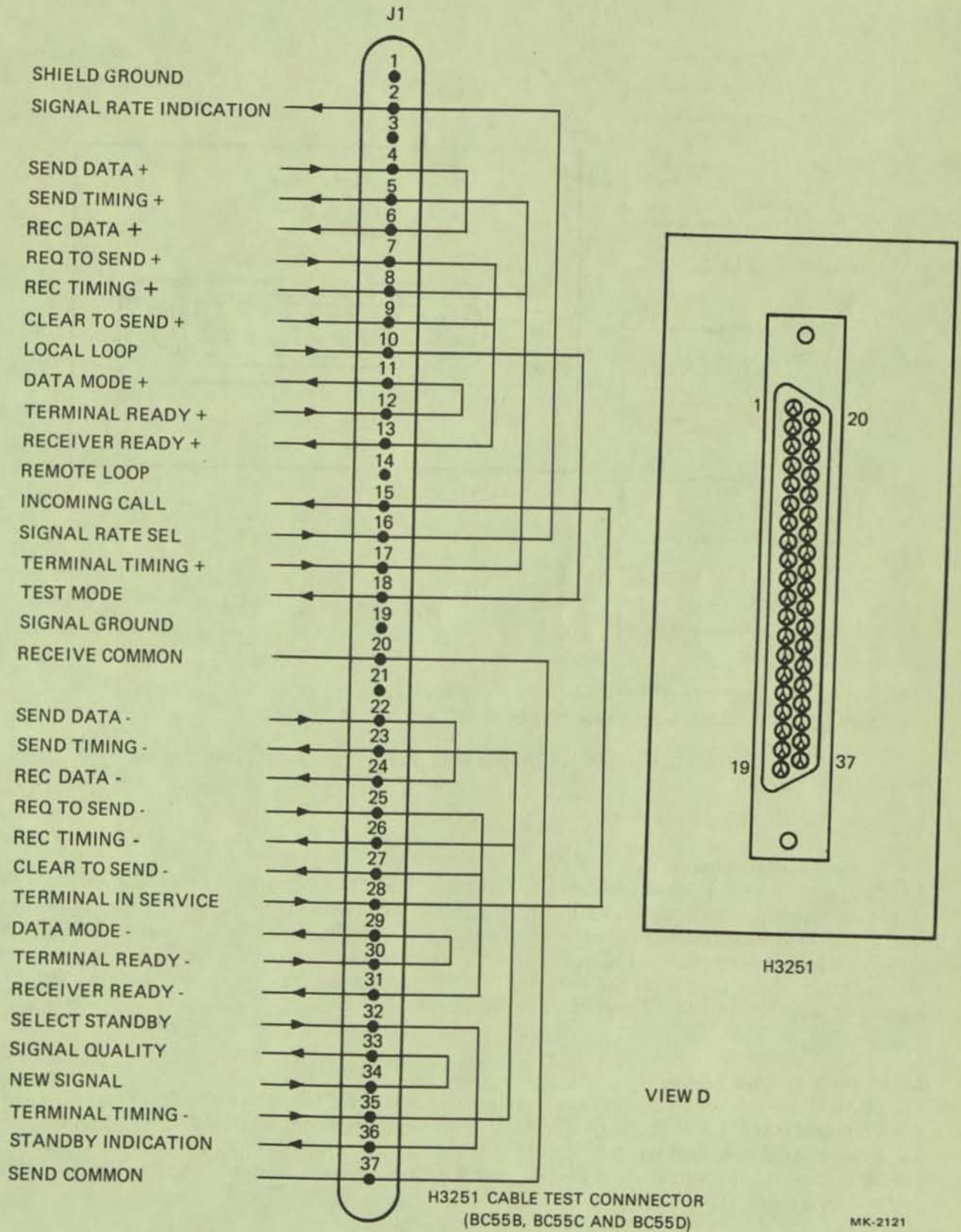
Figure 2-5 DMR11 Turnaround Test Connectors (Sheet 4 of 5)
