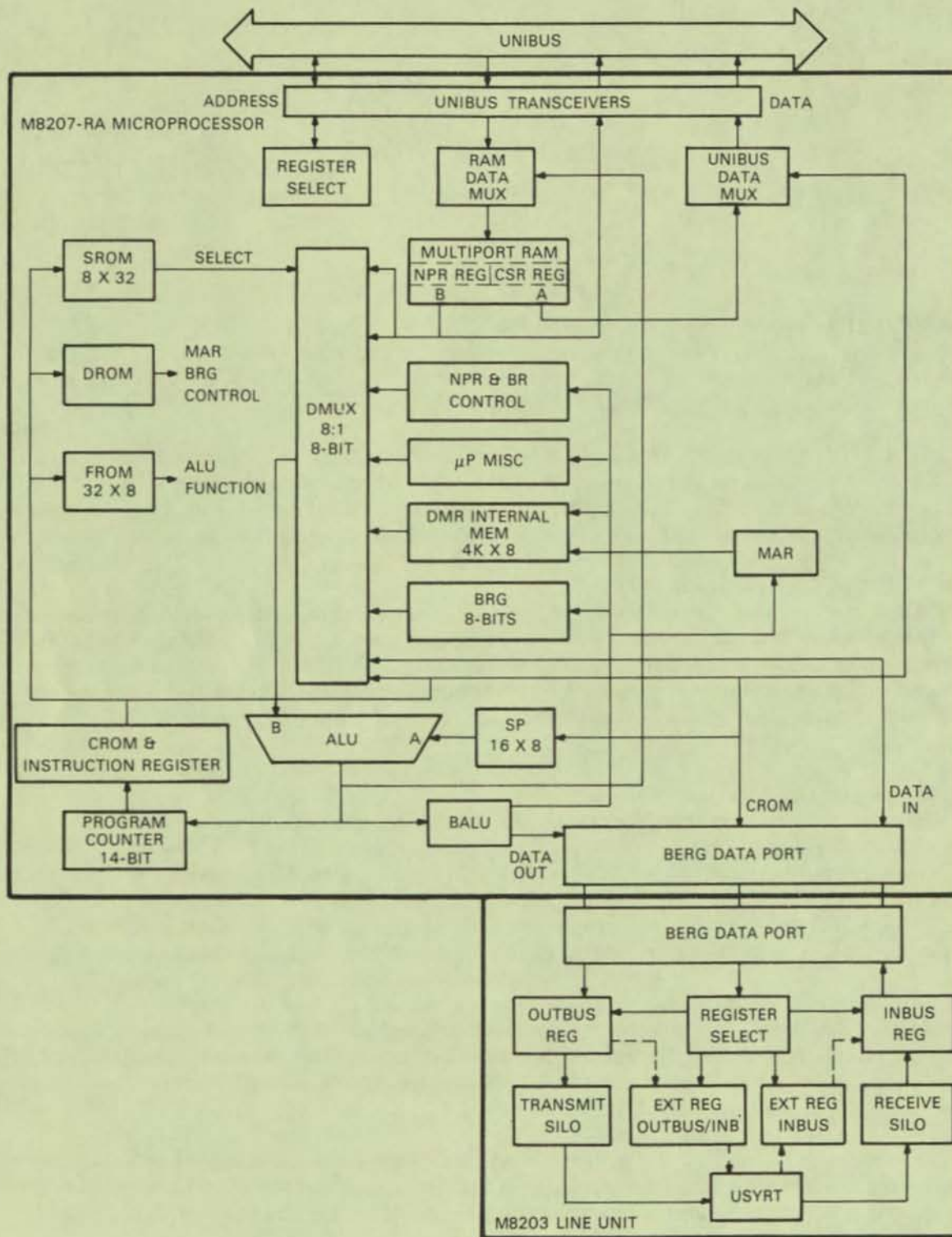
Figure D-1 Data and Control Flow - Basic
