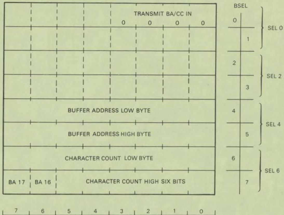
Figure 3-11 Transmit Buffer Address/Character Count In Command Format
