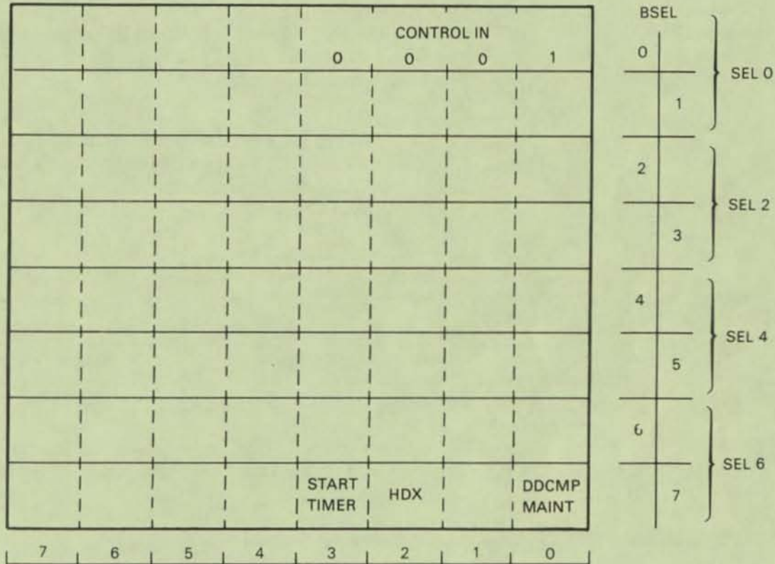
Figure 3-8 Control In Command Format
