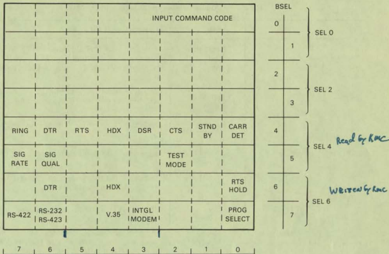
Figure 3-4 Modem Status Read Format
