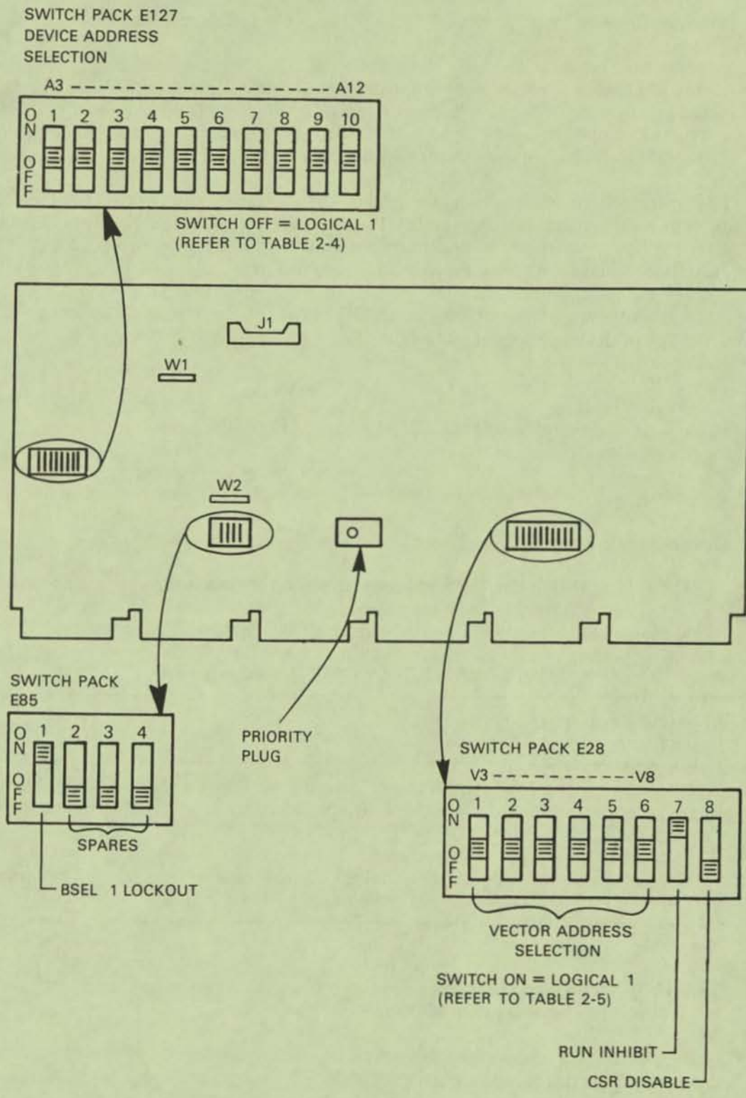
Figure 2-1 M8207-RA Microprocessor Switch/Jumper Locations
