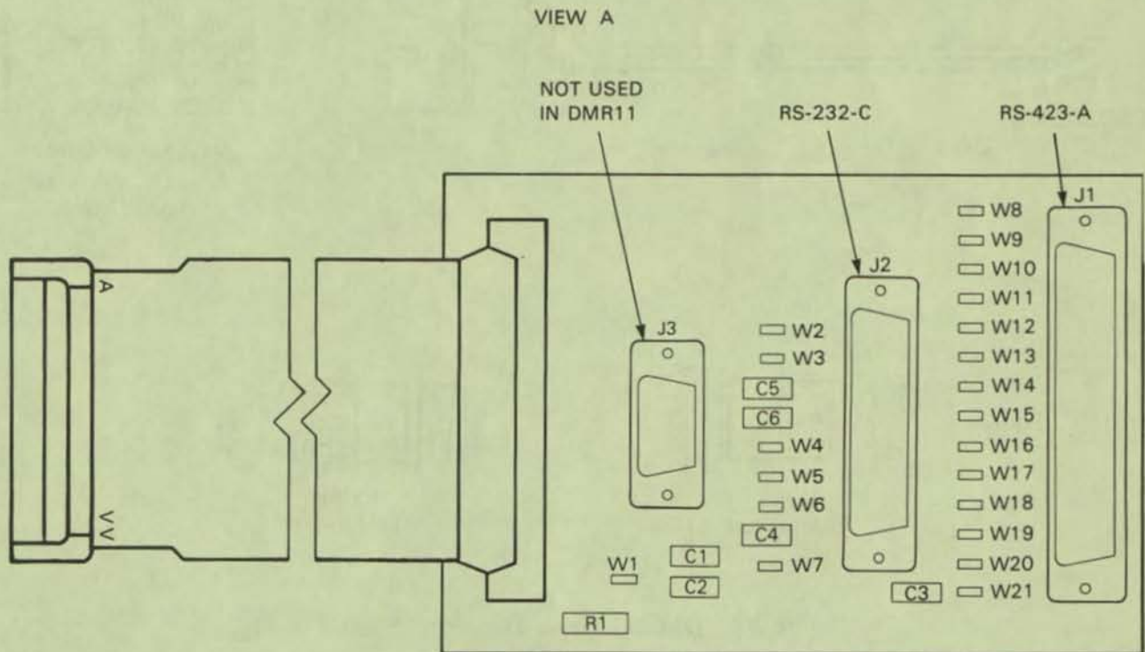
BC55C-10(RS-232-C/RS-423-A) INTERFACE PANEL CABLE
