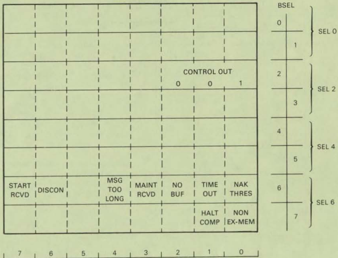
Figure 3-15 Control Out Command Format
