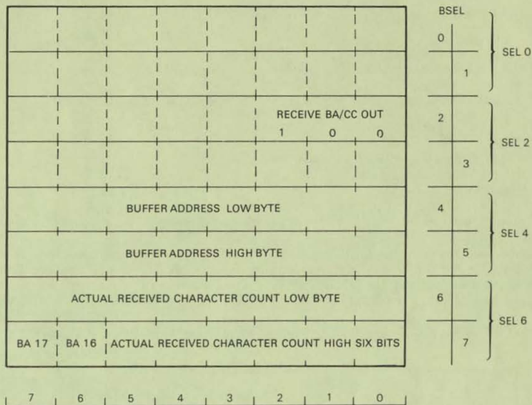
Figure 3-13 Receive Buffer Address/Character Count Out Command Format
