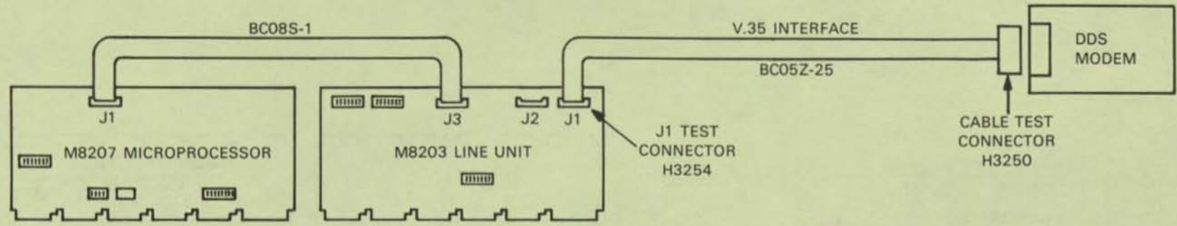
Figure 2-8 DMR-11 REMOTE SYSTEM CABLING
