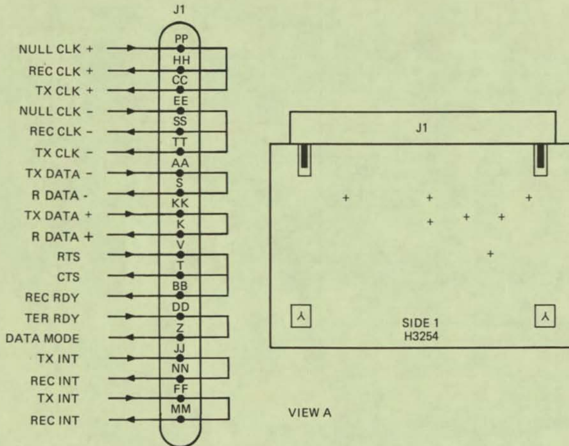
H3254 MODULE TEST CONNECTOR (J1 ON M8203)
