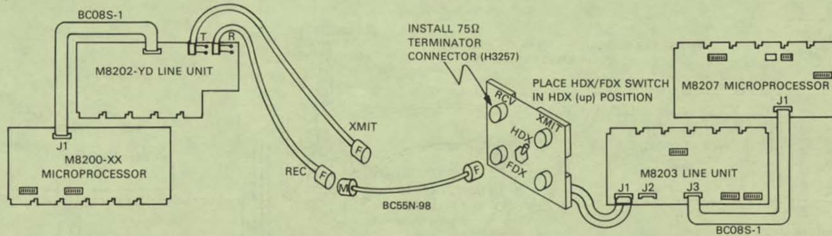
Figure 2-7 DMC11 to DMR11 Integral (Local) Modem Cabling Diagram
