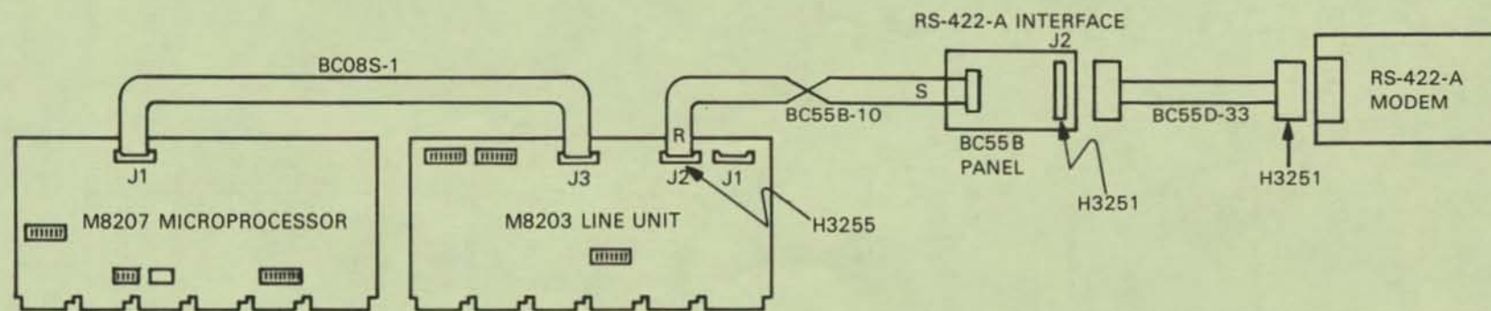
Figure 2-6 DMR11 Remote System Cabling Diagram (Sheet 1 of 2)
