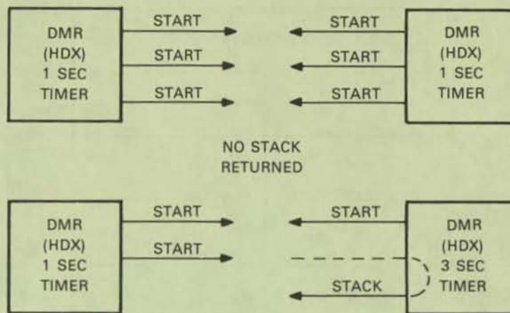
Figure 3-9 Start/Stack Sequence Timer
