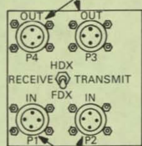
FEMALE CONNECTORS
