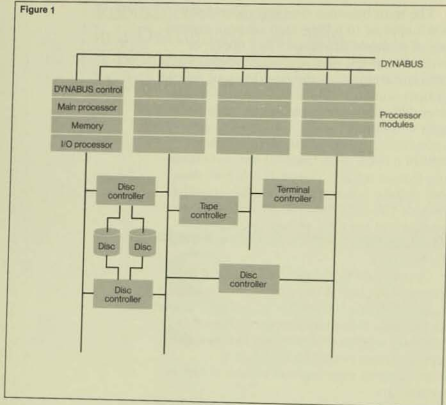
Figure 1. Tandem hardware architecture. A system consists of from 1 to 16 processor modules, each with its own memory, interconnected via the duplexed DYNABUS. The hardware configuration provides redundant paths to the peripherals.
