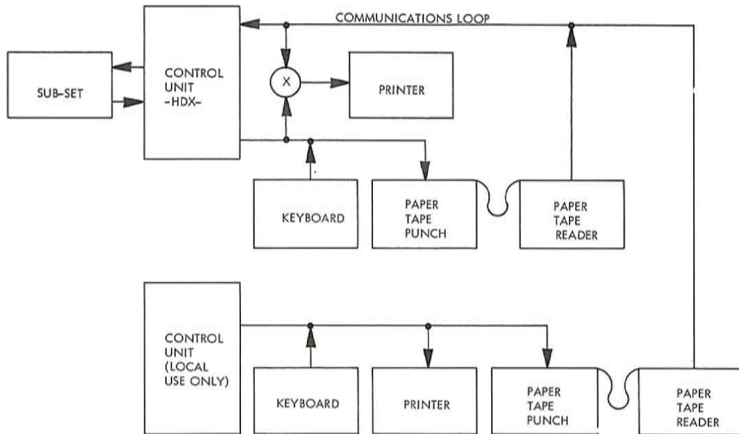
FIGURE 7-6 ACCOUNTING I/O UNIT CONFIGURATION (CONFIG. #4)
