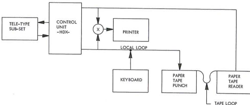
FIGURE 7-12 CONFIGURATION OF I/O UNIT FOR OFF-LINE TRAFFIC OFFICES (CONFIG. #5)
