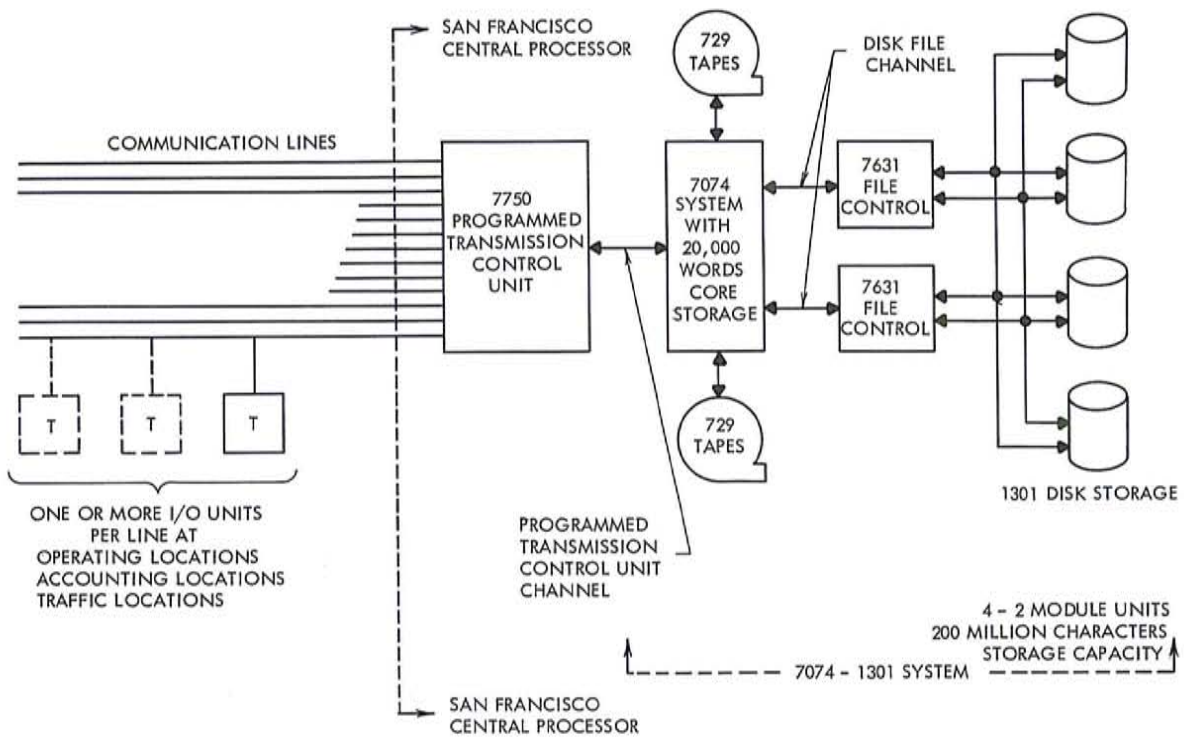
FIGURE 6-1 ON-LINE SYSTEM CONFIGURATION OF THE TOPS SYSTEM
