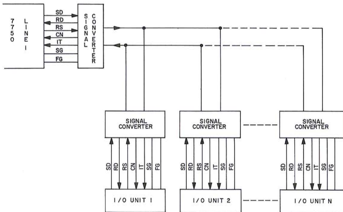
FIGURE 5-2 TYPICAL LINE CONFIGURATION
