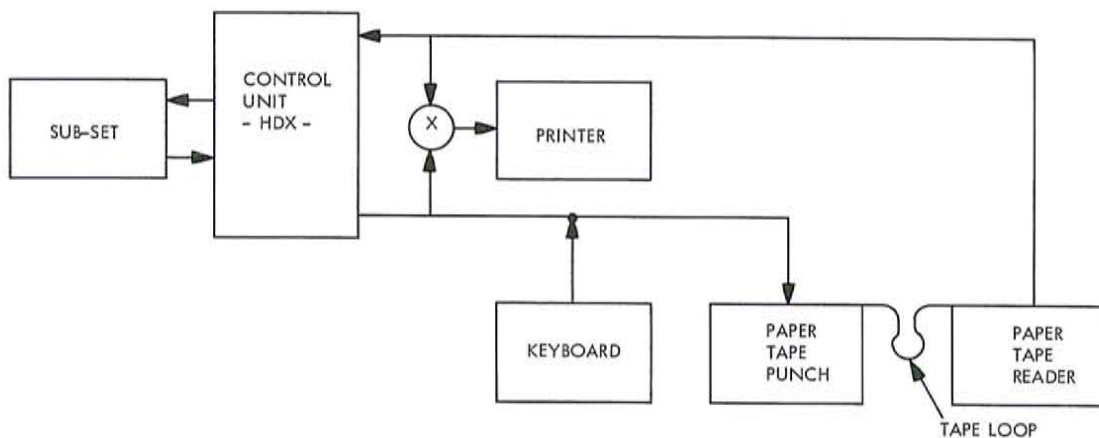
FIGURE 7-8 FREIGHT TRAFFIC, DISPATCHER AND CAR DISTRIBUTOR I/O UNIT CONFIGURATION (CONFIG. #1)
