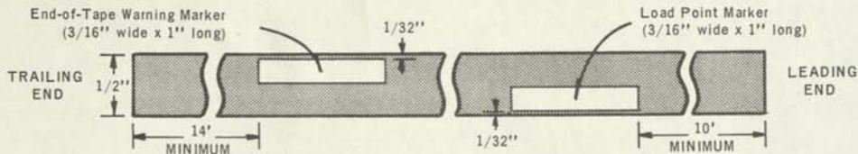
Figure 4-9. Tape Markers
