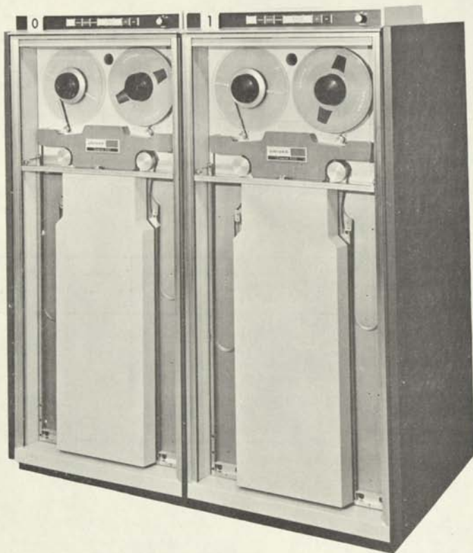
Figure 2-3. UNISERVO VIII C Magnetic Tape Units
