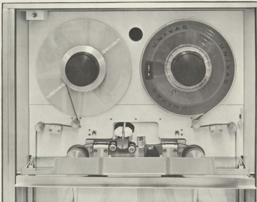
Figure 4-8. Tape Loaded, Leader Attached, and Head Unit Cover Open for Leader Inspection
