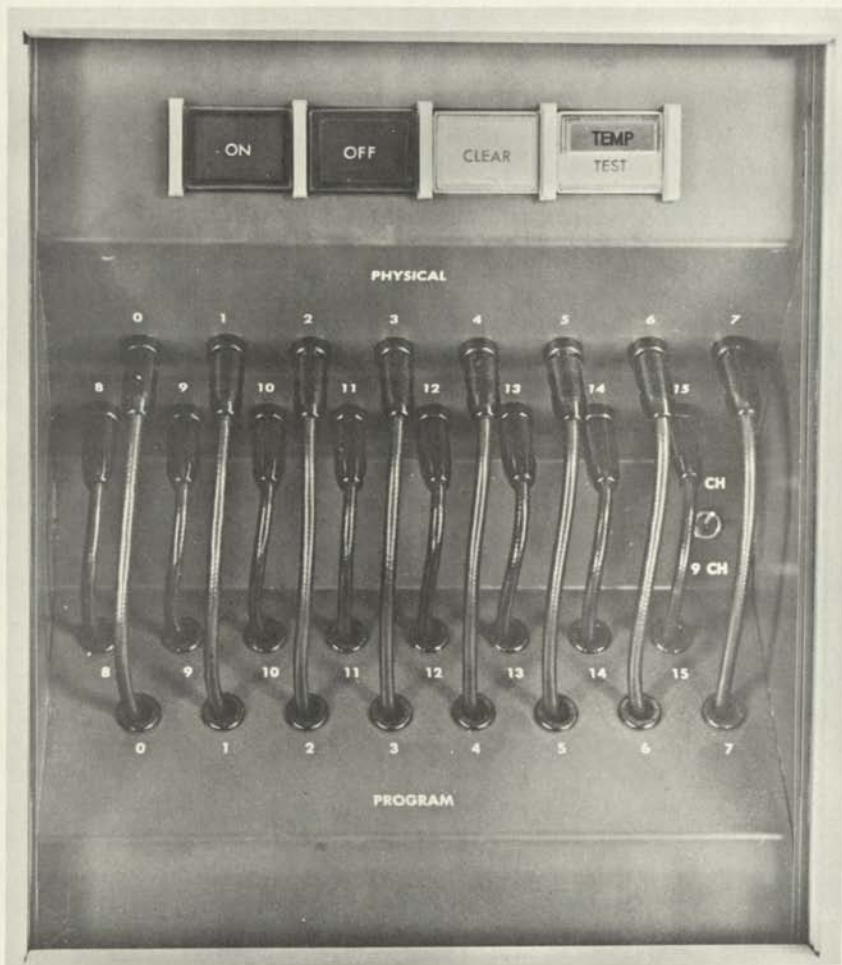
Figure 4-2. Standard Control Unit Control/Indicator Panel
