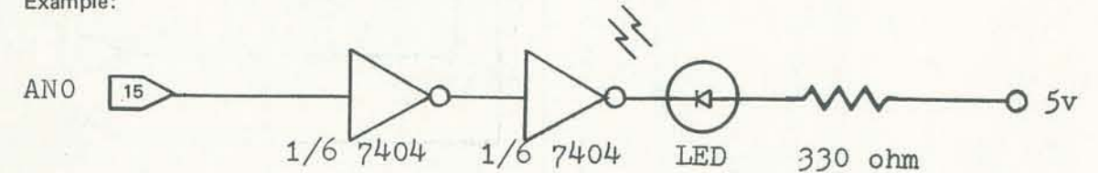
LED Lamp Driver
