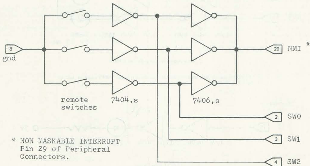
Interrupt Sensing Circuit
