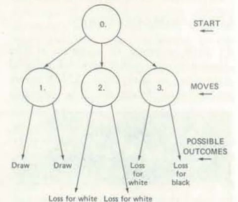
Figure 1. Move Tree Diagram with six outcomes
