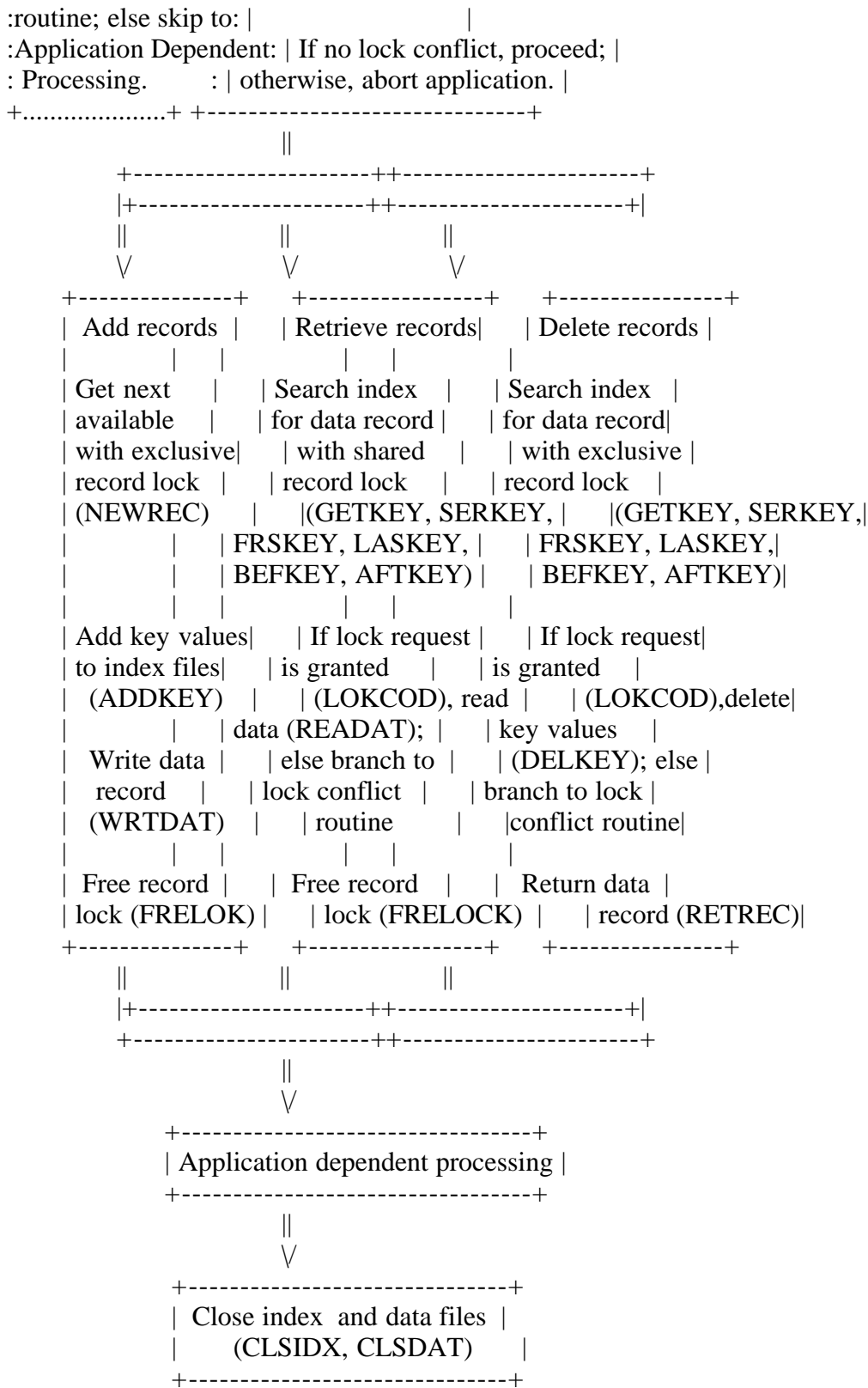
Figure 1-3. Multiuser program flow
