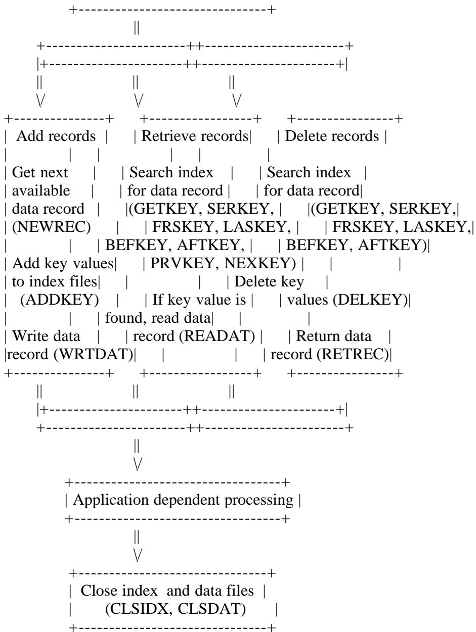
Figure 1-2. Single-user program flow
