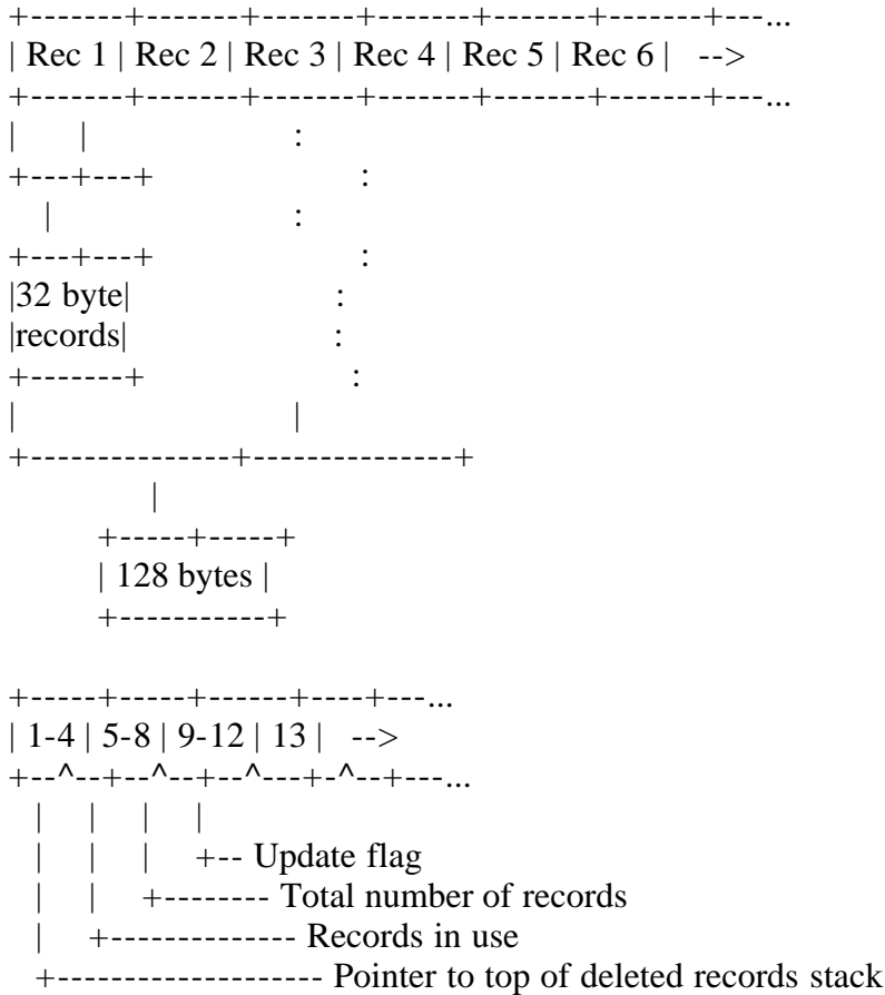
Figure 3-2. Sample data file layout for 32-byte records
