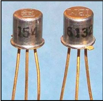
Transistor Size (1/8" OD X 3/16") Standard TO-18 Date Code 6132 (1963 Week 32)
