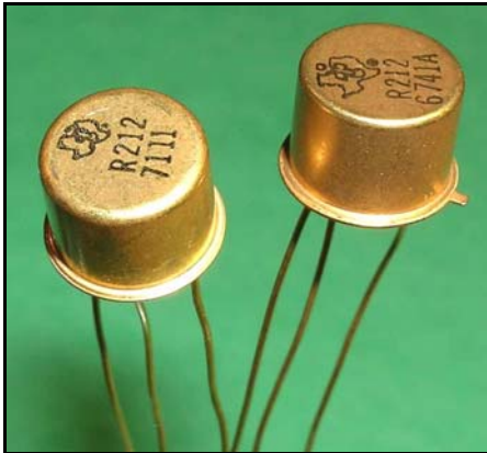
Transistor Size (1/4" Diameter X 1/4"H) Standard TO-5 Case Date Codes 7111 (1971) and 6741A (1967)
