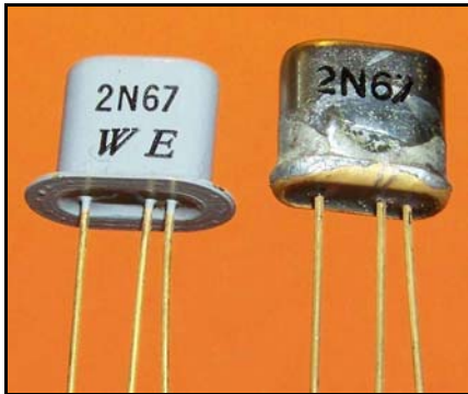
Transistor Size (1/2" L X 1/8"W X 5/16" H) Date Code on Right Unit 450 (1954, Week 50) Date Code on Left Unit 652 (1956, Week 52)
