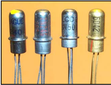
Transistor Size (1/8" OD X 3/8") Classic "Bullet-Shaped" TO-24 Typical Date Code 6042 (1960 Month 42)
