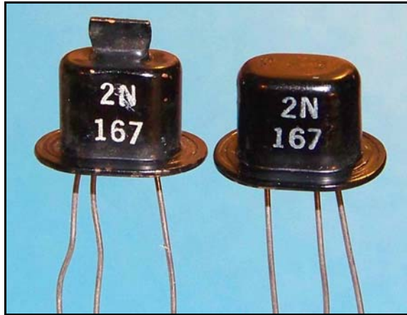
Transistor Size (1/2" L X 1/4"W X 1/2" H) "Bath-Tub" Oval Case Date Code on Left Unit 048 (1960, Week 48) No Date Code on Right Unit
