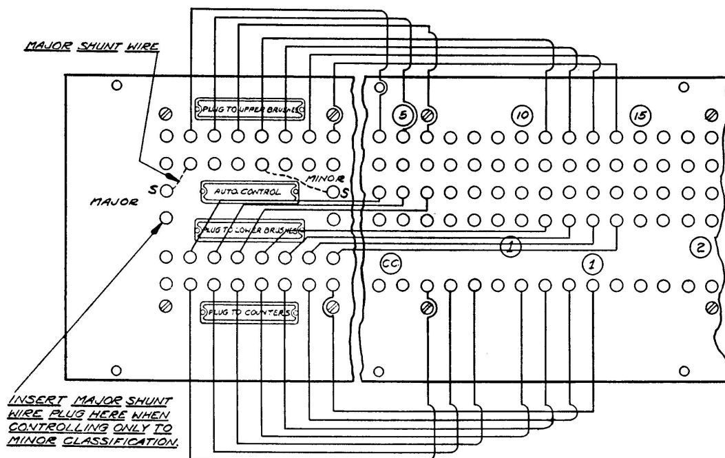
PLUGBOARD OF AUTOMATIC-CONTROL TABULATOR
