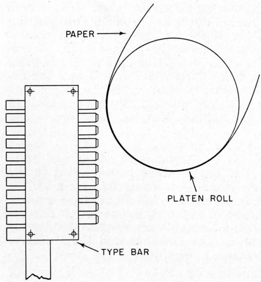
Relative Positions of Type Bar and Platen
